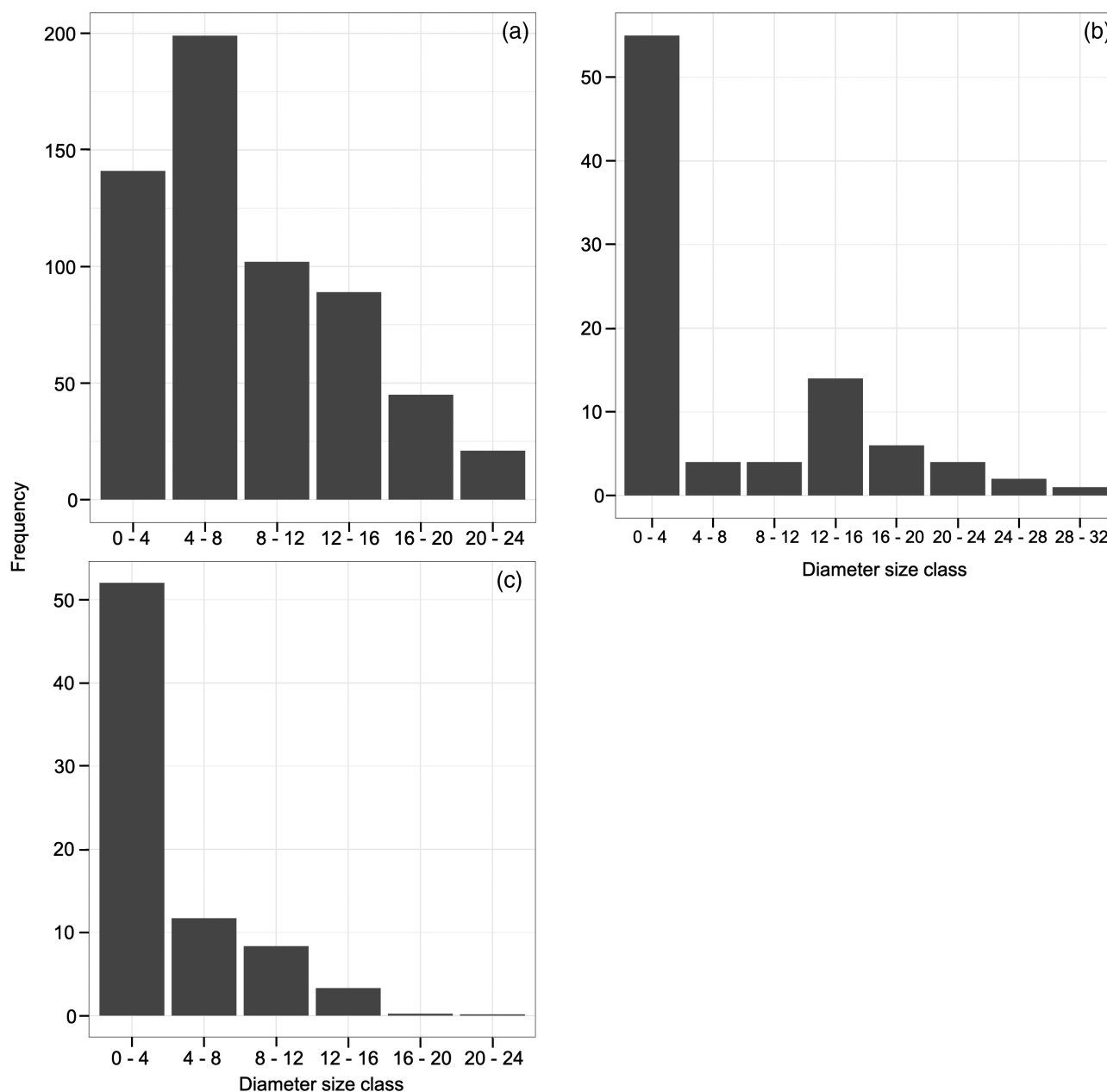
FIGURE 4 Diameter size class distribution for the three most common wild climber species harvested for food harvesting, processing and storage products around Bwindi: (a) Smilax anceps , (b) Monanthes littoralis , and (c) Dracaena laxissima
