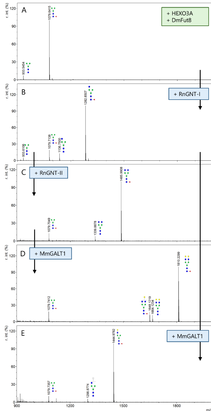
Figure 5. MALDI-TOF MS spectra of PNGase F glycans generated on OoASP-1 through combining in planta and in vitro glycoengineering. N. benthamiana plants were infiltrated with A. tumefaciens strains harboring expression constructs for OoASP-1, NbHEXO3A and DmFUT8 to obtain OoASP-1 with Man 3 GlcNAc 2 Fuc glycans ( A ). Subsequent in vitro glycoengineering with RnGNT-I, RnGNT-II and MmGALT1 was performed to generate pharmaceutically relevant native OoASP-1 glycans ( B , C , D , E ). Green boxes depict constructs used for in planta glycoengineering, blue boxes depict enzymes used for in vitro glycoengineering. Black arrows indicate sequential in vitro reactions. Peaks that could not be labeled to glycans are left unannotated. Glycan structures are drawn according to symbol nomenclature for glycans (SNFG).
