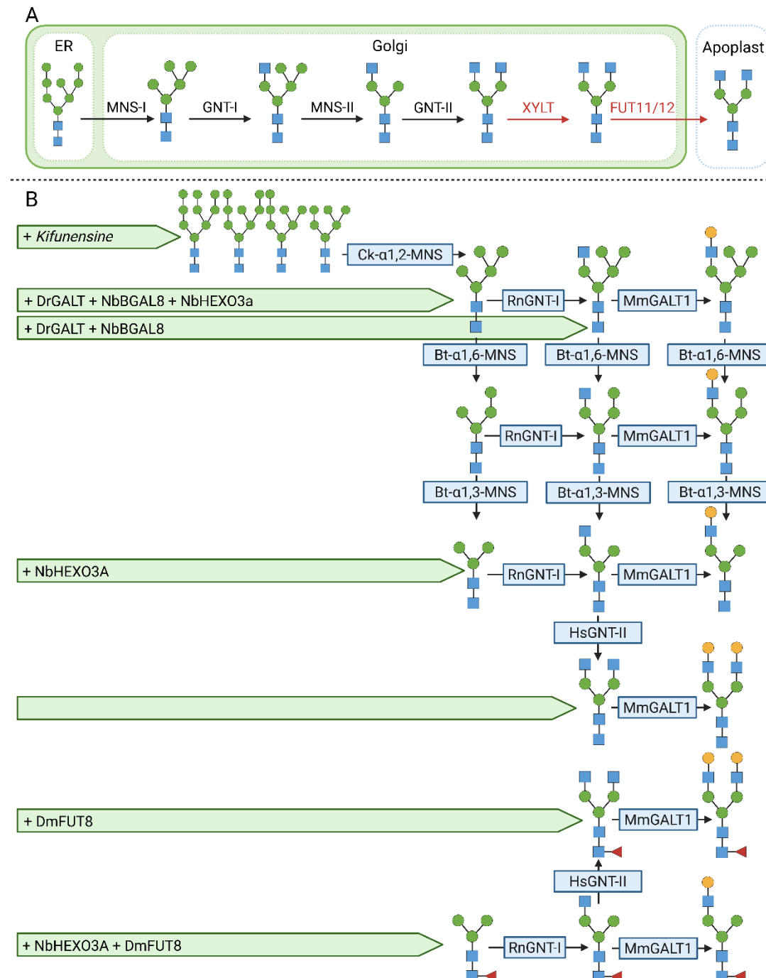
Figure 1. In planta and in vitro glycan processing pathways. A General glycan processing pathway of the N. benthamiana XT/FT plant line. B Glycan processing pathways than can be achieved through combining in planta and in vitro glycoengineering. Green arrows represent chemicals ( italics ) or glycoenzyme-encoding plasmids in A. tumefaciens that are infiltrated into N. benthamiana XT/FT plants to facilitate in planta glycoengineering. Arrows with blue blocks indicate E.coli produced enzymes that are used for in vitro glycoengineering reactions. Glycan structures are drawn according to symbol nomenclature for glycans (SNFG). Created in BioRender .
