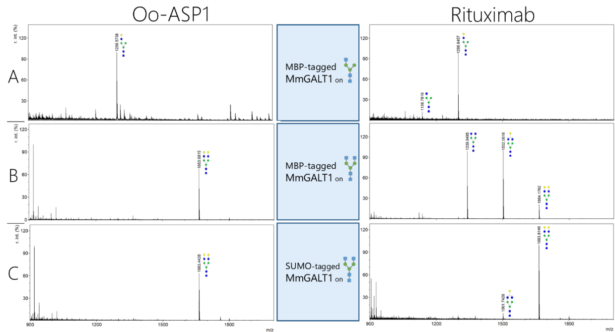
Figure 3. MALDI-TOF MS spectra of PNGase F released glycans generated on OoASP-1 and Rituximab through in vitro galactosylation by SUMO and MBP-tagged MmGALT1. In vitro glycoengineered OoASP-1 and Rituximab, containing GlcNAcMan 3 GlcNAc 2 and GlcNAcMan 5 GlcNAc 2 glycans, were galactosylated by SUMO and MBP-tagged MmGALT1 as depicted in the blue boxes. Peaks that could not be labeled to glycans are left unannotated. Glycan structures are drawn according to symbol nomenclature for glycans (SNFG).
