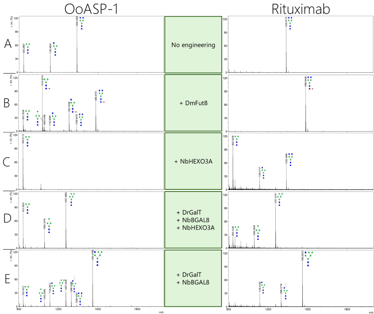
Figure 4. MALDI-TOF MS spectra of PNGase F released glycans generated on OoASP-1 and rituximab through in planta glycoengineering. N. benthamiana plants were infiltrated with A. tumefaciens strains harboring expression constructs for OoASP-1 (left column) or rituximab (right column), together with strains harboring expression constructs for relevant glycosyltransferases or glycosidases (depicted in middle column). Each row (A-E) represents a different glycoengineering strategy. Peaks that could not be labeled to glycans are left unannotated. Glycan structures are drawn according to symbol nomenclature for glycans (SNFG).
