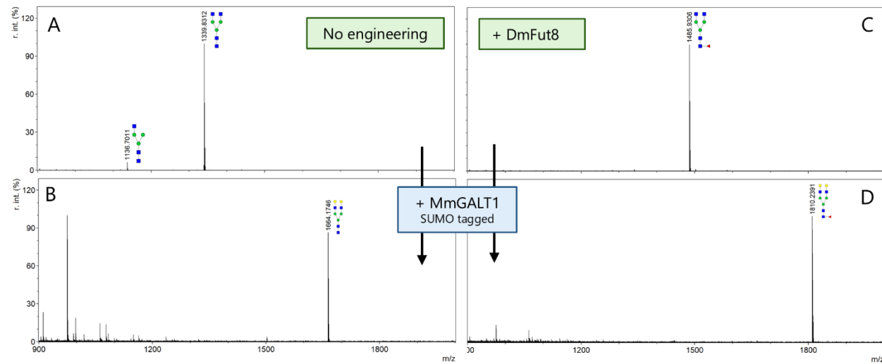
Figure 6. MALDI-TOF MS spectra of glycans generated on rituximab through combining in planta and in vitro glycoengineering. N. benthamiana plants were infiltrated with A. tumefaciens strains harboring expression constructs for rituximab and DmFut8 to obtain GlcNAc 2 Man 3 GlcNAc 2 and GlcNAc 2 Man 3 GlcNAc 2 Fuc glycans ( A and B , respectively). Both substrates were then modified in vitro with SUMO-tagged HsGALT1 to facilitate galactosylation ( C and D ). Green boxes depict constructs used for in planta glycoengineering, blue boxes depict enzymes used for in vitro glycoengineering. Black arrows indicate sequential in vitro reactions. Peaks that could not be labeled to glycans are left unannotated. Glycan structures are drawn according to symbol nomenclature for glycans (SNFG).
