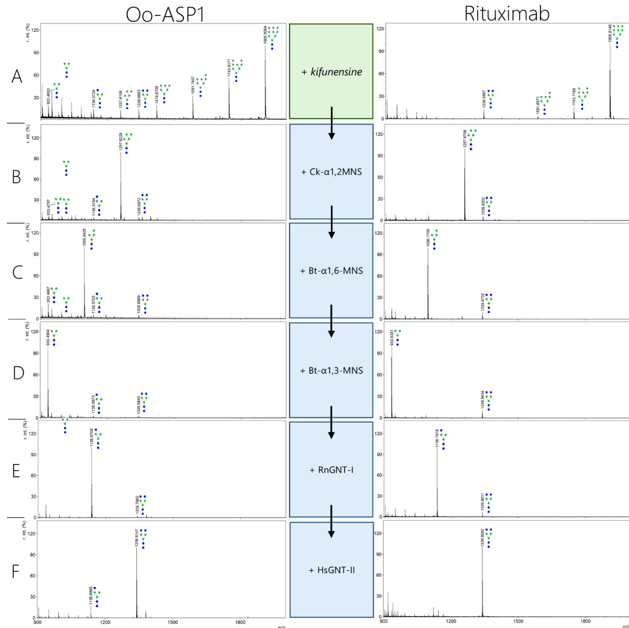
Figure 2. MALDI-TOF MS spectra of PNGase F released glycans generated on OoASP-1 and Rituximab through sequential in vitro glycoengineering. Plant-produced high-mannose OoASP-1 and Rituximab (Green box, A ) were sequentially modified to reach a biantennary GlcNAc using E. coli -expressed glycoenzymes (Blue boxes, B-F ). Black arrows indicate sequential in vitro reactions. Peaks that could not be labeled to glycans are left unannotated. Glycan structures are drawn according to symbol nomenclature for glycans (SNFG).
