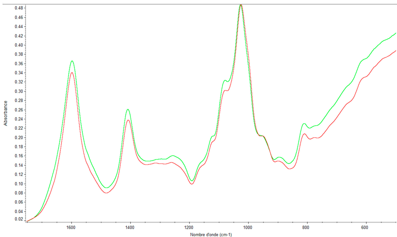
Figure 12. FTIR spectra of soluble Sargassum muticum alginates collected in February (green spectrum) and June (red spectrum).
