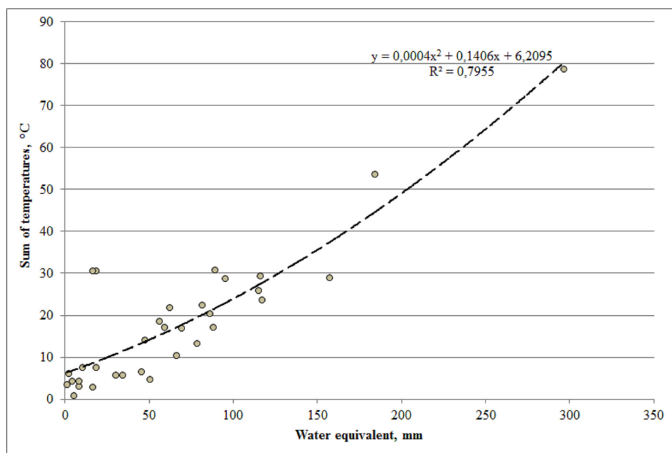
Figure 2. The dependence of snow cover melting on the sums of positive average daily air temperatures along the snow courses of weather station Zmeinogorsk from year 2013 to year 2021.
