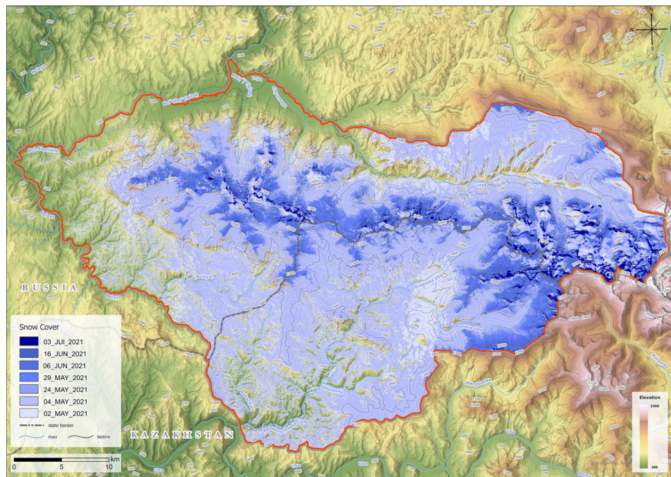
Figure 4. Position of snow cover on the Tigiretsky Range on specific dates in 2021.
