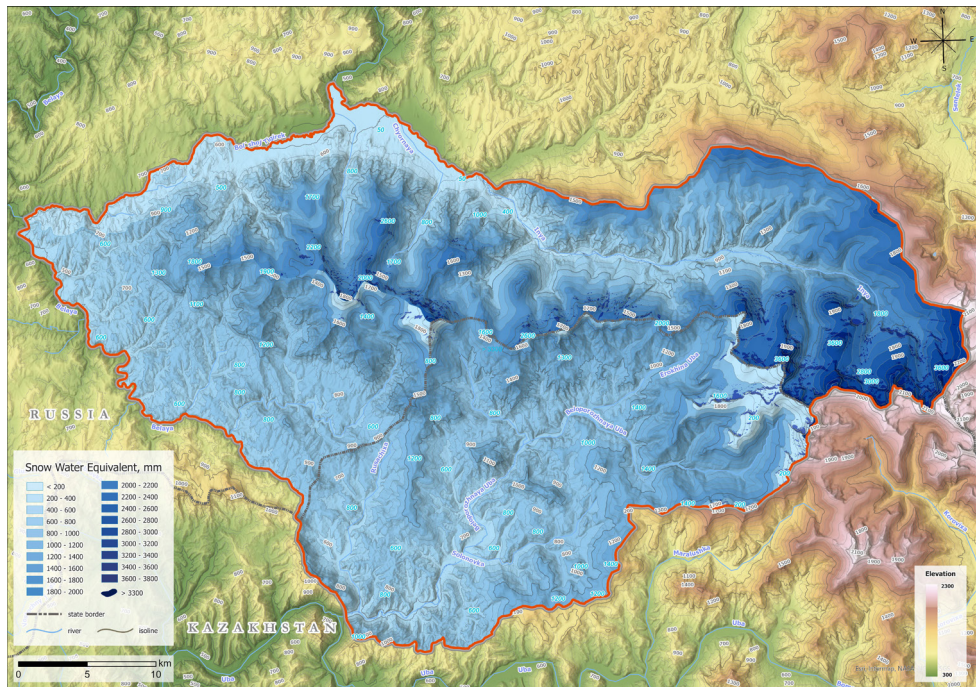
Figure 5. Maximum water content of snow cover on the Tigiretsky Range (Altai) in winter 2020–2021.
