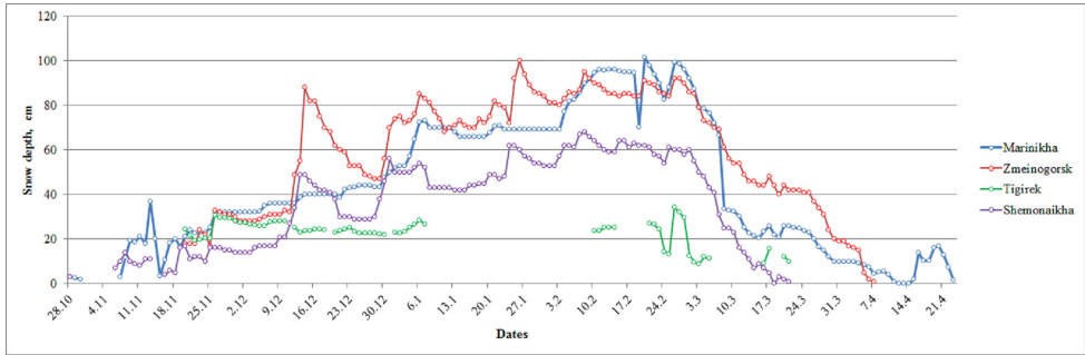
Figure 1. Snow depth (cm) during the winter period of 2022–2023 at weather stations in Zmeinogorsk (Russia), Shemonaikha (Kazakhstan), and observation sites of the Tigirek Nature Reserve (Russia) at the Tigirek and Marinikha cordons.
