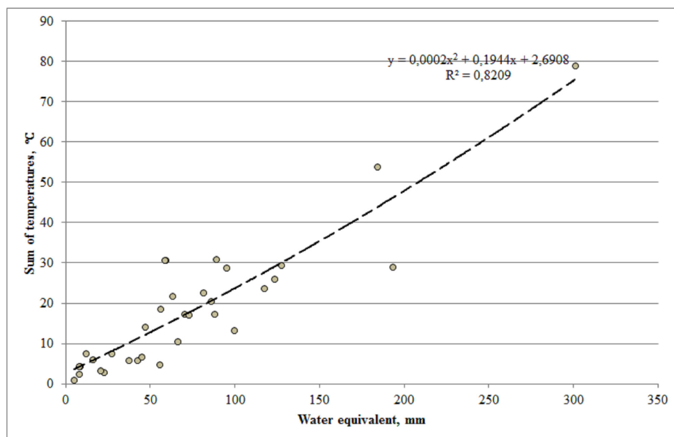
Figure 3. The dependence of snow cover melting on the sums of positive average daily air temperatures along the snow courses of weather station Zmeinogorsk from year 2013 to year 2021, taking into account the precipitation that occurred during periods of negative air temperatures.
