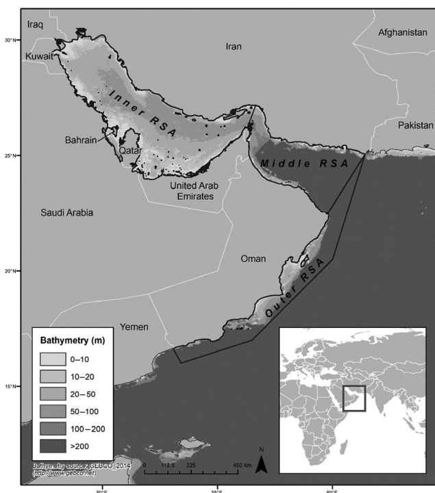
FIGURE 1 Map of the study (risk assessment) area, the Regional Organization for Protection of the Marine Environment (ROPME) Sea Area showing the Inner and Middle Sea Areas which were the focus of this study
