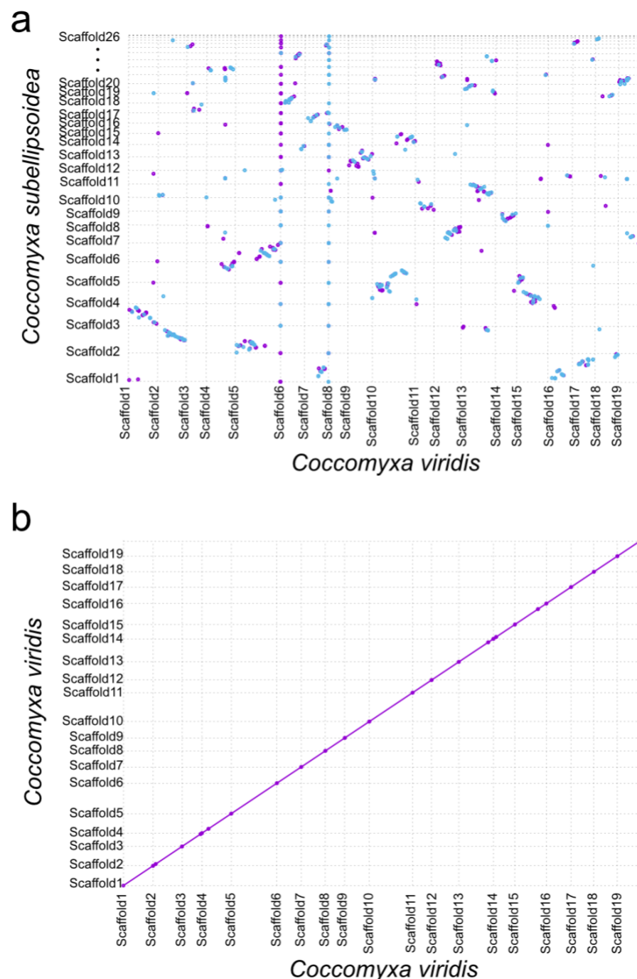
Figure 5. No syntenicity detected between related Coccomyxa species. (a) Dot plot of orthologous sequences in the genome assemblies of C. viridis SAG 216-4 and C. subellipsoidea C-169. Violet and blue dots represent orthologous sequences on same and opposite strands, respectively. Dot sizes does not correlate with the length of the sequences they represent, which were all < 1 kb. The width of each box corresponds to the length (bp) of the respective scaffold. (b) Dot plot of the genome assembly of C. viridis SAG216-4 against itself.
