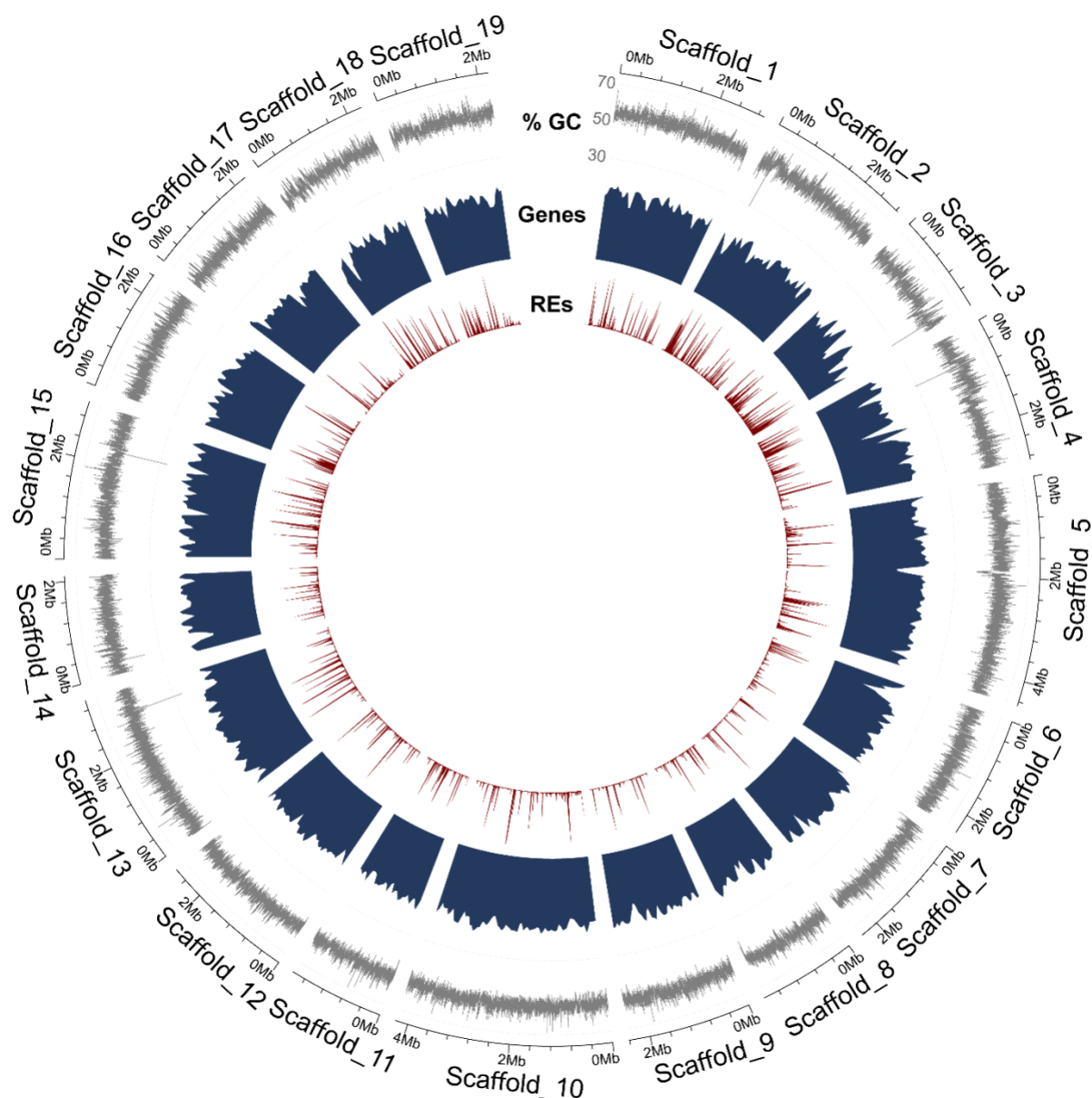
Figure 4. Circos plot summarizing the nuclear genome annotation of Coccomyxa viridis SAG 216-4. From outside to inside the tracks display: GC content (over 1-kb windows), gene density (blue) and repetitive element density (red).
