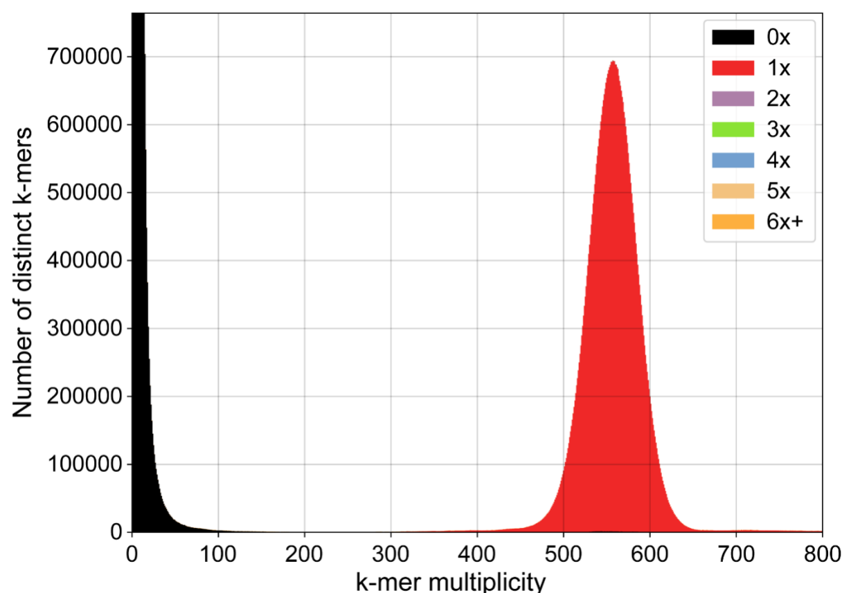
Figure 3. The Coccomyxa viridis SAG 216-4 genome is haploid. The KAT spectra-cn plot depicts the 27-mer multiplicity of the PacBio HiFi reads against the genome assembly. Black areas under the peaks represent k-mers present in the reads but absent from the assembly, colored peaks indicate k-mers that are present once to multiple times in the assembly. The single red peak in the KAT spectra-cn plot suggests that Coccomyxa viridis has a haploid genome, while the black peak at low multiplicity shows that the assembly is highly complete and that all reads are represented in the assembly.
