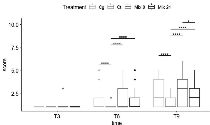
FIGURE 1 General effect of different treatments on anthracnose disease score in yam over time. Cg, inoculation of strain from Colletotrichum gloeosporioides complex; Ct, inoculation of strain from C. truncatum complex; Mix 0, inoculation of initial admixture; Mix 24, sequential inoculation (strain from C. truncatum complex inoculated 24 h prior to strain from C. gloeosporioides complex). The effect is averaged for the two C. gloeosporioides strains. **** p < 0.0001 , * p < 0.05 . Dots represent experimental values occurring outside confidence interval.
