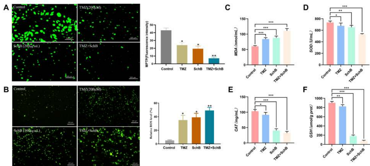
Fig. 3. Effect of TMZ/Sch B combination on the mitochondrial function of U87 cells. (A) MPTP staining evaluates mitochondrial permeability transition pore opening. Scale bar = 100 μm. (B) ROS levels measured by DCFH-DA staining. Scale bar = 100 μm. (C) Lipid peroxidation assessed via MDA content. (D–F) Antioxidant enzyme activities of SOD, CAT, and GSH, respectively. Data are presented as mean ± SD. * p < 0.05, ** p < 0.01, and *** p < 0.001. MPTP, Mitochondrial Permeability Conversion Pore; ROS, reactive oxygen species; SOD, superoxide dismutase; CAT, catalase; GSH, glutathione.
