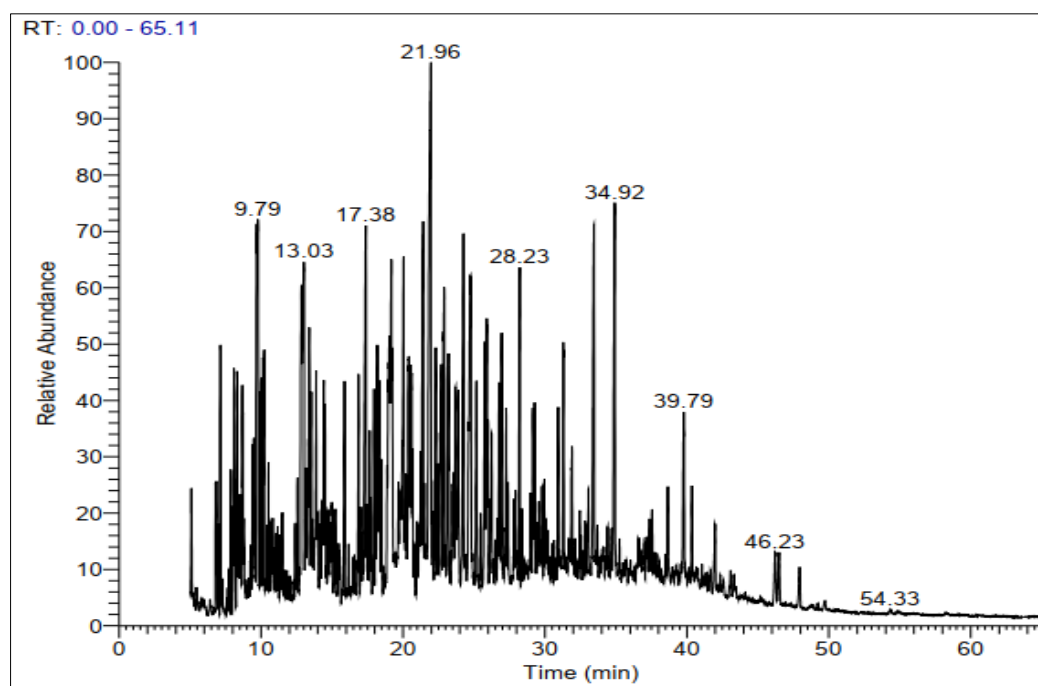
Figure 2. Representative GC-MS chromatogram of derivatized methanolic extract of C. mixtus leaves.
