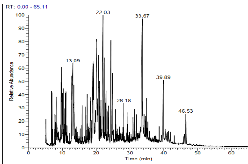
Figure 3. Representative GC-MS chromatogram of derivatized methanolic extract of C. mixtus stems.
