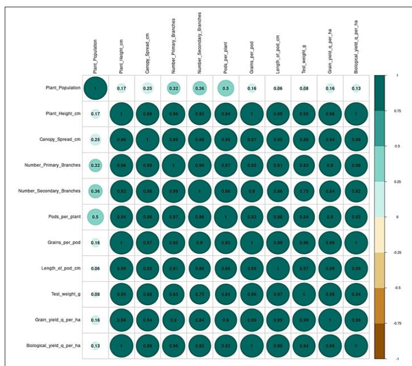
Fig 3: Correlogram analysis of growth and yield traits under system of intensification and organic mulching in pigeon pea.
