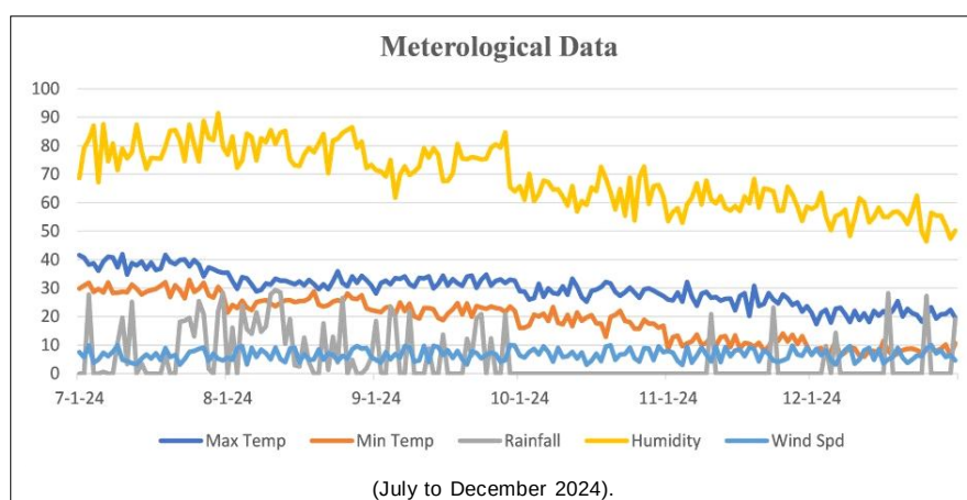
Fig 2: Mean standard meteorological data weather parameters and total rainfall during the cropping season.
