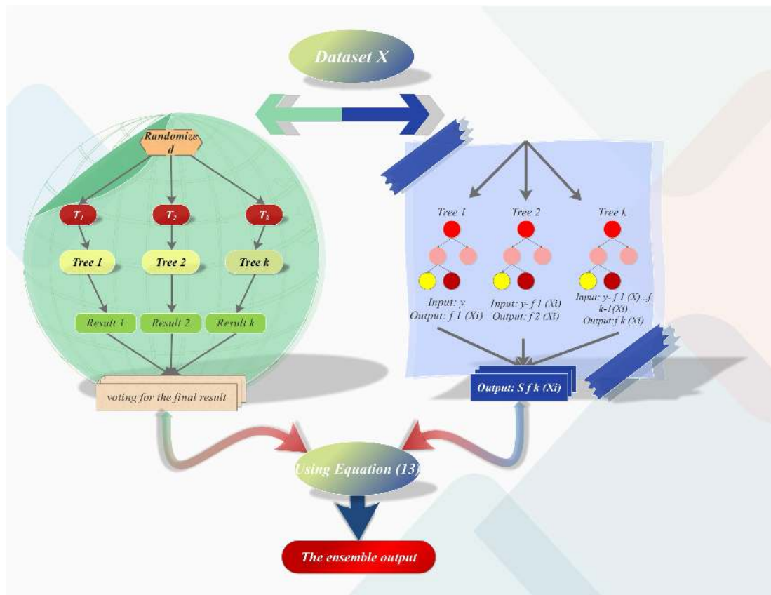
Figure 11: The procedure of presented ensemble models
