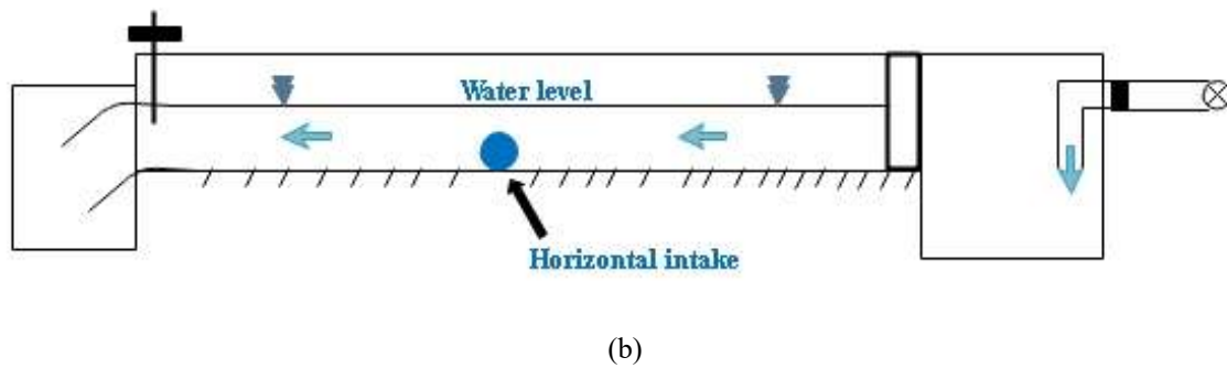
Figure 1: Experimental setup [24], a) plan, b) elevation
