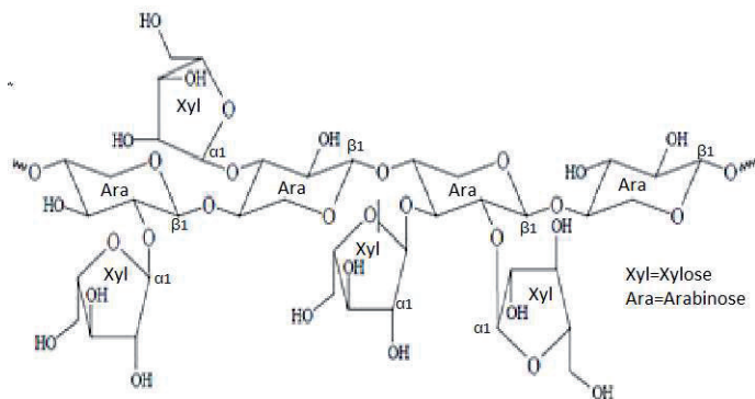
Figure 1. Arabinoxylan structure.
