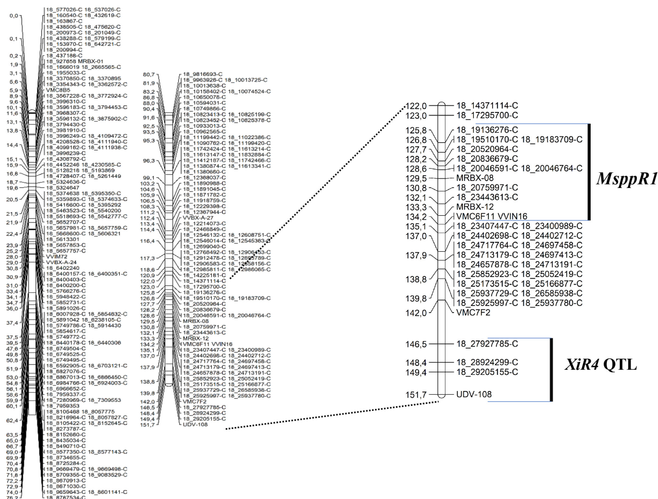
FIGURE 3. Location of the RKN MsppR1 locus on the chromosome 18 (shown in two parts) of VRH8771. Genetic distances in cM are displayed on the left-hand side and marker names (SNP and SSR markers) are displayed on the right-hand side. The detailed map shows the region encompassing MsppR1 (this study) and the XiR4 QTL for resistance to X. index (Rubio et al. , 2020).
