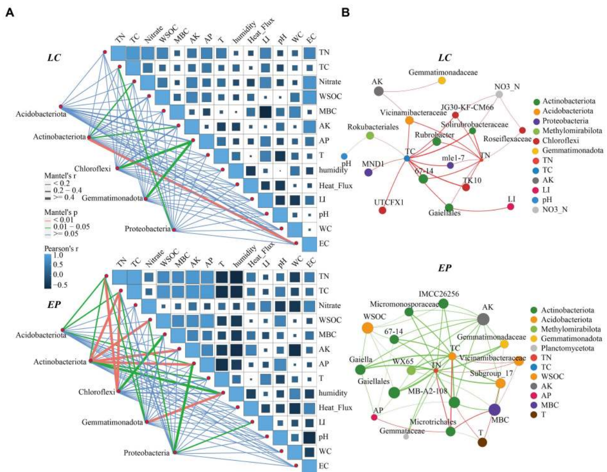
FIGURE 6 (A) Correlation analysis and the Mantel test of soil properties and dominant SBCs in the genus LC and EP plots; (B) Two-factor correlation network analysis of core genera (Degree > 30) and environmental factors in the EP and LC plots; TC, total carbon; TN, total nitrogen; WSOC, water-soluble organic carbon; MBC, microbial carbon; AK, available potassium; AP, available phosphorus; EC, electric conductivity. LI, Light Intensity.
