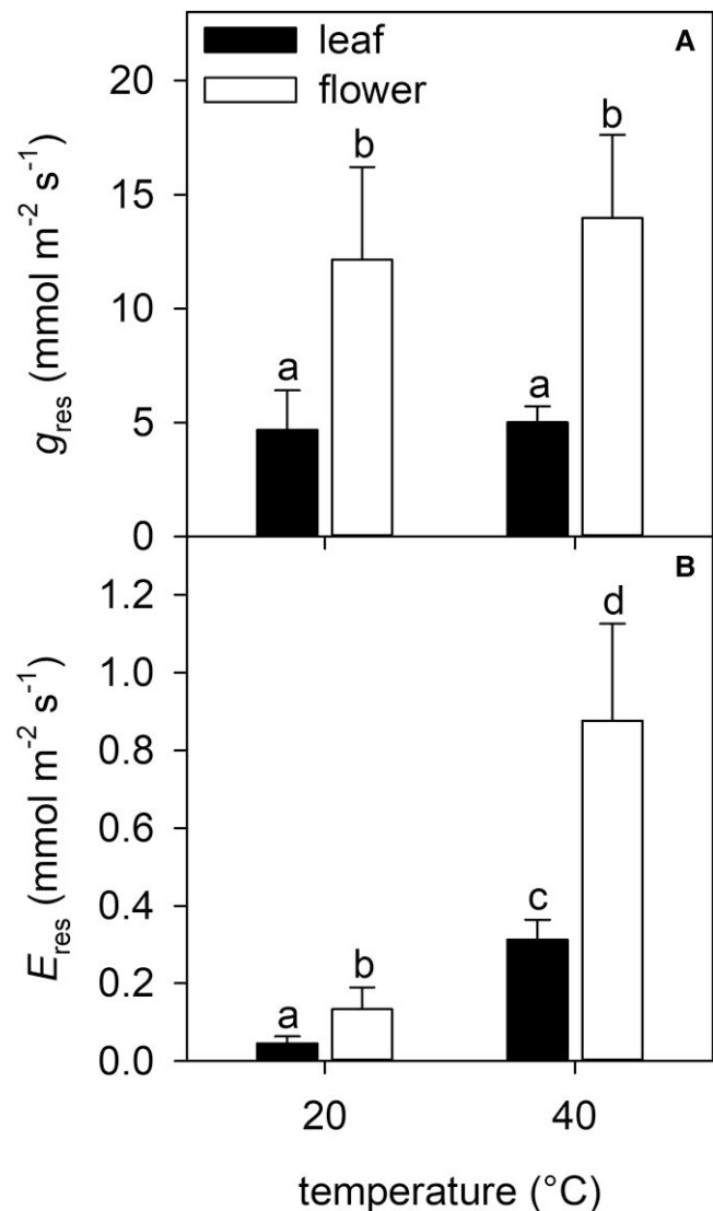
Figure 1. Pyrethrum flowers have greater conductance to water vapor after stomatal closure than leaves at both 20 and 40°C. Residual conductance to water vapor ( g_{\text{res}} ) A , and transpiration ( E_{\text{res}} ) B at 20 and 40°C of leaves and flowers exposed to water stress predicted to close stomata. Columns are means + SE ( n = 3 individuals). Different letters indicate significant differences among means: a-b and c-d ( P < 0.05 ), a-c and b-d ( P < 0.001 ) ( g_{\text{res}} : organ F_{1,8} = 9.922 , P < 0.05 ; temperature F_{1,8} = 0.401 , P > 0.05 ; organ:temperature F_{1,8} = 0.001 , P > 0.05 ) ( E_{\text{res}} : organ F_{1,8} = 8.954 , P < 0.05 ; temperature F_{1,8} = 29.646 , P < 0.001 ; organ:temperature F_{1,8} = 1.685 , P > 0.05 ).
