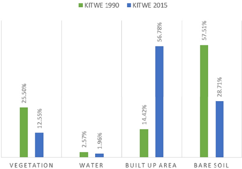
Figure 4. Land use and land cover changes in Kitwe between 1990 and 2015.
