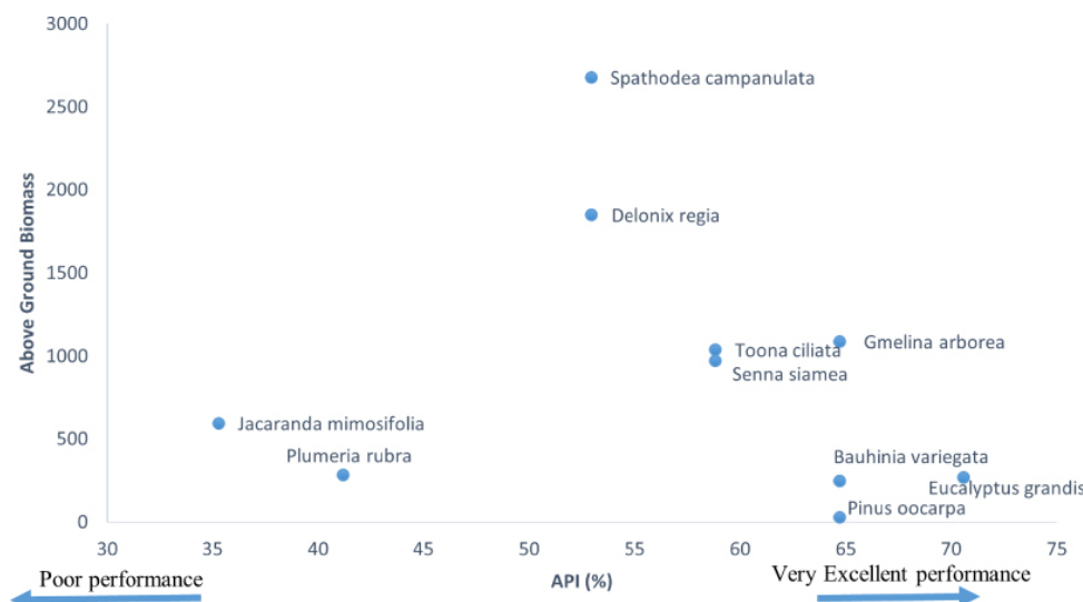
Figure 15. Comparison between tree species AGB and API.
