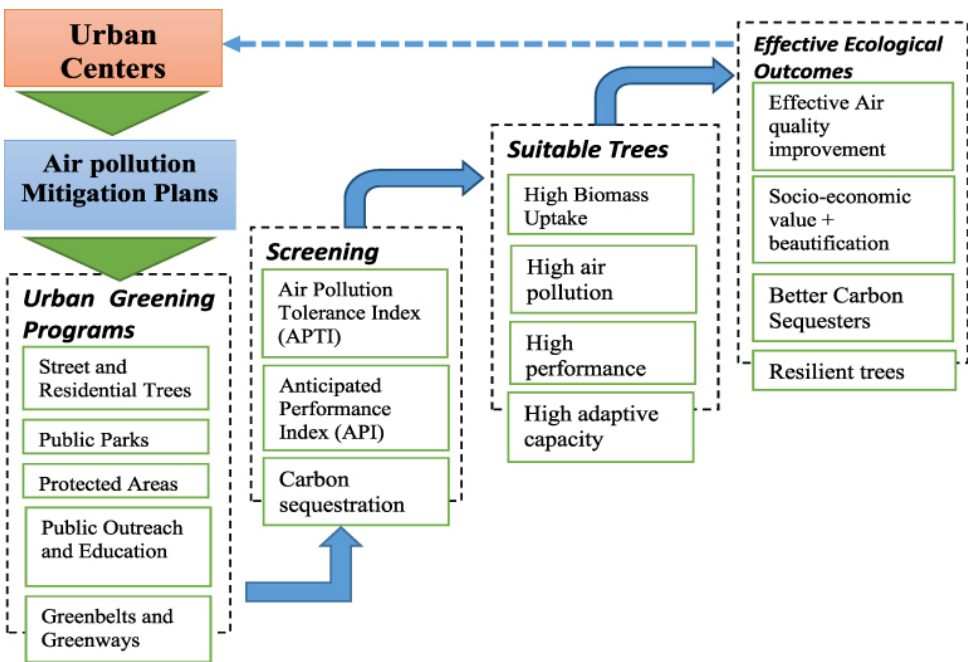
Figure 3. Conceptual framework for identification of urban greening suitable plants.
