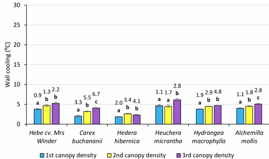
Fig. 2 Mean wall panel cooling (°C) by different taxa when the control wall panel temperature is 25 °C. Numbers above the bars are WLAI and lines on the bars denote +/- standard errors. Different letters note the significant difference between the mean values of a taxon
