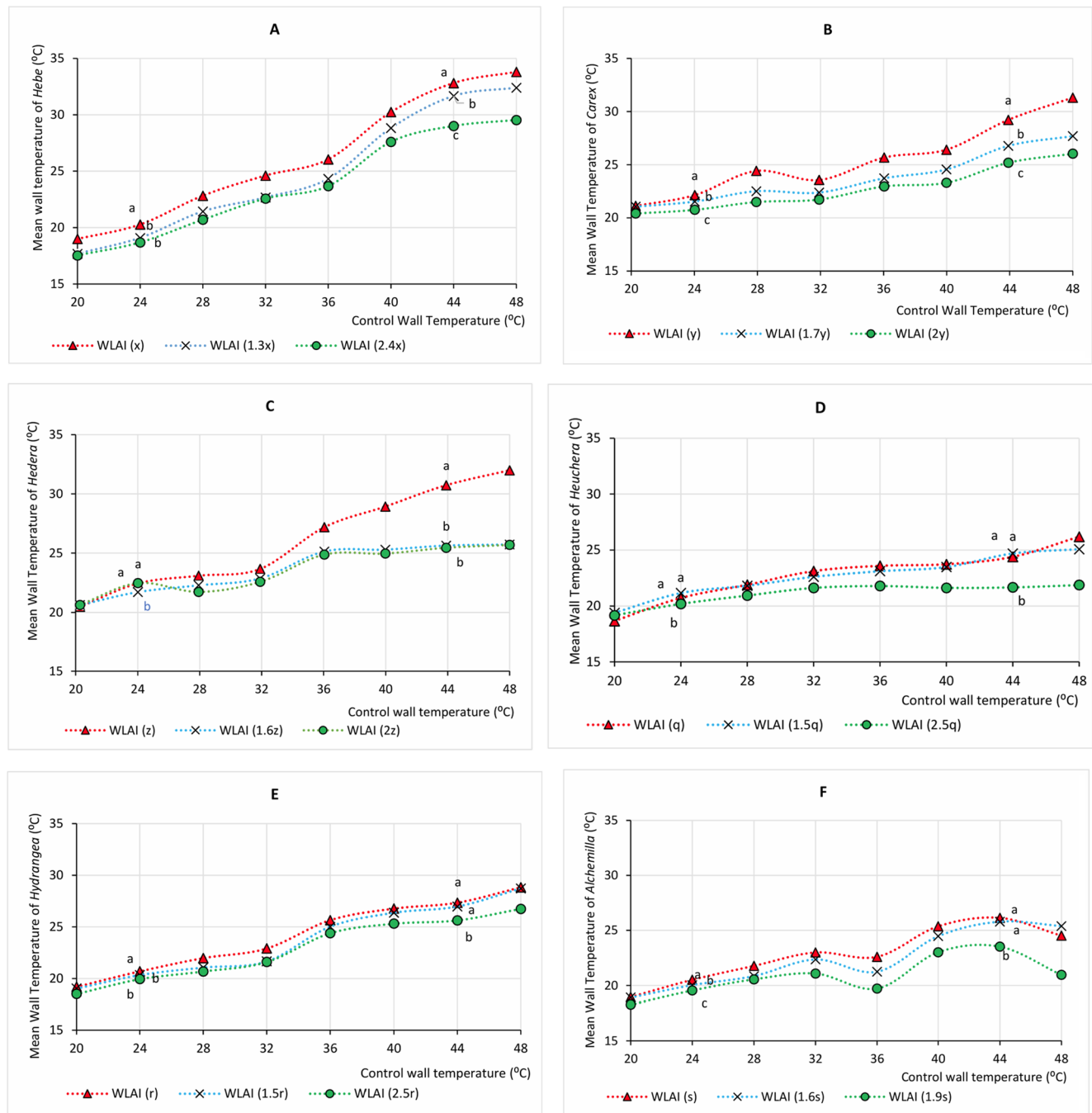
Fig. 4 Comparison of wall panel temperature (°C) between levels of canopy coverage in various taxon – Hebe (A), Carex (B), Hedera (C), Heuchera (D), Hydrangea (E), and Alchemilla (F). Different letters denote significant differences in the trend line at control temperatures of 24 and 44 °C
