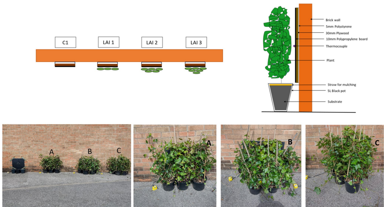
Fig. 1 Top view diagram (Top left) shows plant positioning in front of wall panels (Plants are green with different canopy coverage in front of the wall panels i.e. LAI1, LAI2, and LAI3 and a non-planted control – C1). The wall is depicted in brown, and the insulated panels are black. Side view (Top right) of individual panel setup of LAI1 with plant spacing (Kunasingam et al. 2024). The bottom image shows the experimental setup (with Hedera hibernica in this case) in a wide range (left) and a close-up of planting arrangements of three different canopy width levels A- LAI1, B- LAI2, and C- LAI3 (right). Note a white vinyl cloth used to stop thermal gain in the black pots has been removed to show the position of the plants
