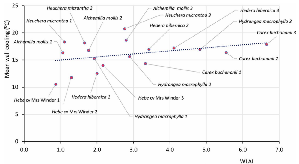
Fig. 5 The relationship between WLAI and wall panel cooling (mean of all temperatures (°C)). Correlations explained 10% ( r^2=0.10 ) of the variance
