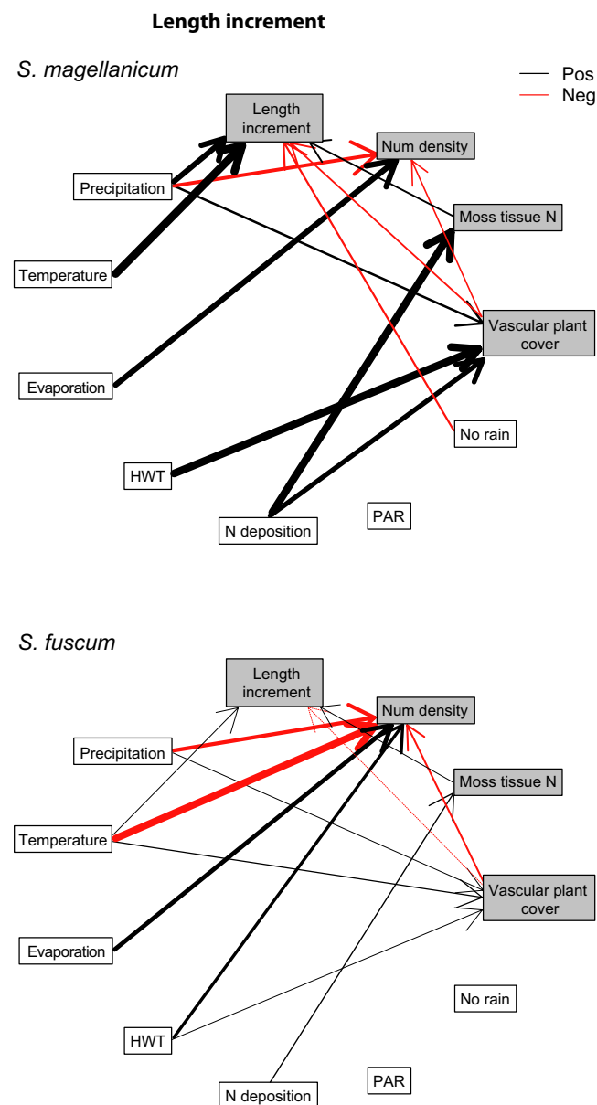
FIGURE 5 Graphical representation of piecewise structural equation models using mixed effects models to describe effects of the environmental variables from the models in Table S4 on annual length increment. Num density = numerical density of Sphagnum shoots, PAR = photosynthetic active radiation, No rain = mean length of rain free periods, HWT = height above the water table. White boxes are exclusively predictor variables, grey boxes are response (length increment), or predictor and response. Arrowheads show the direction of effects and line thickness indicates the effect size. For simplicity, arrows associated with p \geq 0.1 have been removed. See Table S7 for complete model results
