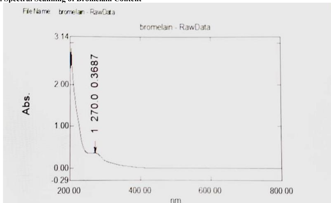
Graph 1: Absorption spectrum of Bromelain at 270 nm
