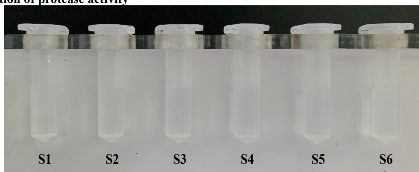
Fig 11: protease assay of standard tyrosine at different concentrations
