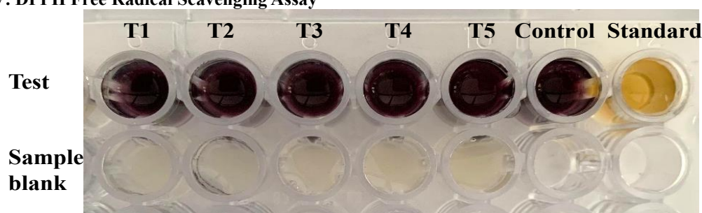
Fig 13: DPPH Free Radical Scavenging Assay of sample with standard and control
