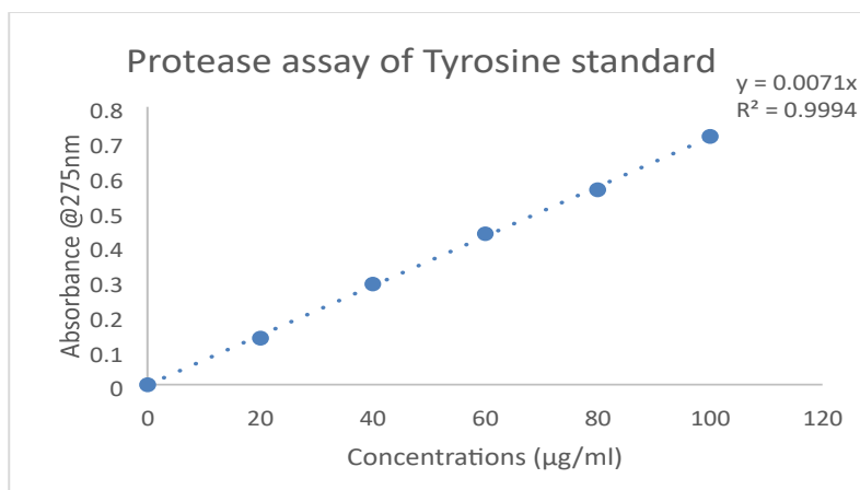
Graph 2: protease assay of standard tyrosine at different concentrations
