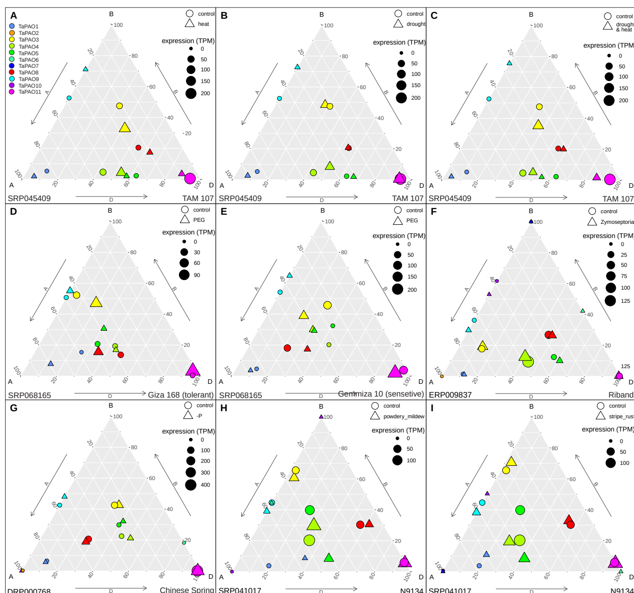
Supplementary Fig. S1. Ternary plot showing relative expression abundance of TaPAO genes under different stress conditions. In each ternary plot, a circle or a triangles reflects the relative contribution of homoeologs of a gene under normal or stress condition, respectively and their sizes indicate the total expression in TPM. The data code for each study and the evaluated wheat cultivar are also indicated at bottom of subfigures.
