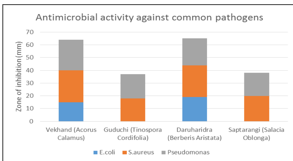
Fig. no. 4: Comparison of growth inhibition shown by each plant extracts against pathogens.
