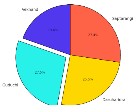
DPPH Scavenging Activity (%) of Different Samples
