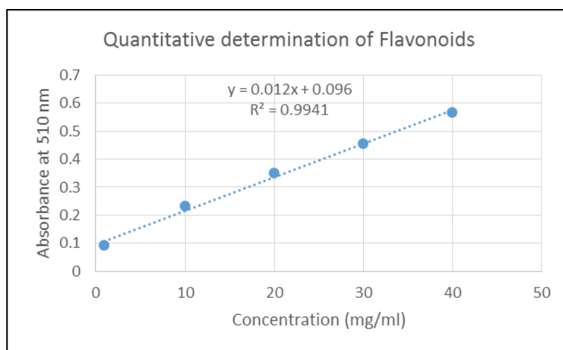
Fig.no. 1: Standard graph of flavonoids.
