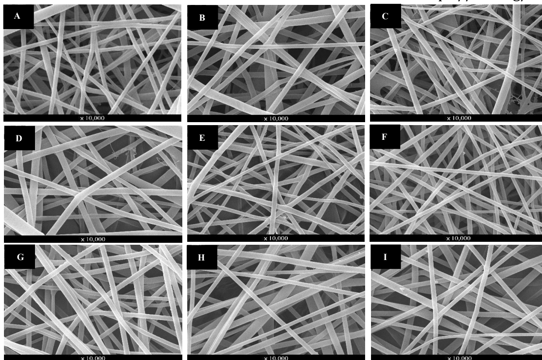
Figure 7 Morphologies of PVA: RJ extract nanofibers at a 7:3 ratio under (a) 30 kV, (b) 35 kV, and (c) 45 kV; at 8:2 ration under (d) 30 kV, (e) 35 kV, and (f) 45 kV; and at a 9:1 ratio under (g) 30 kV, (h) 35 kV, and (i) 45 kV.
