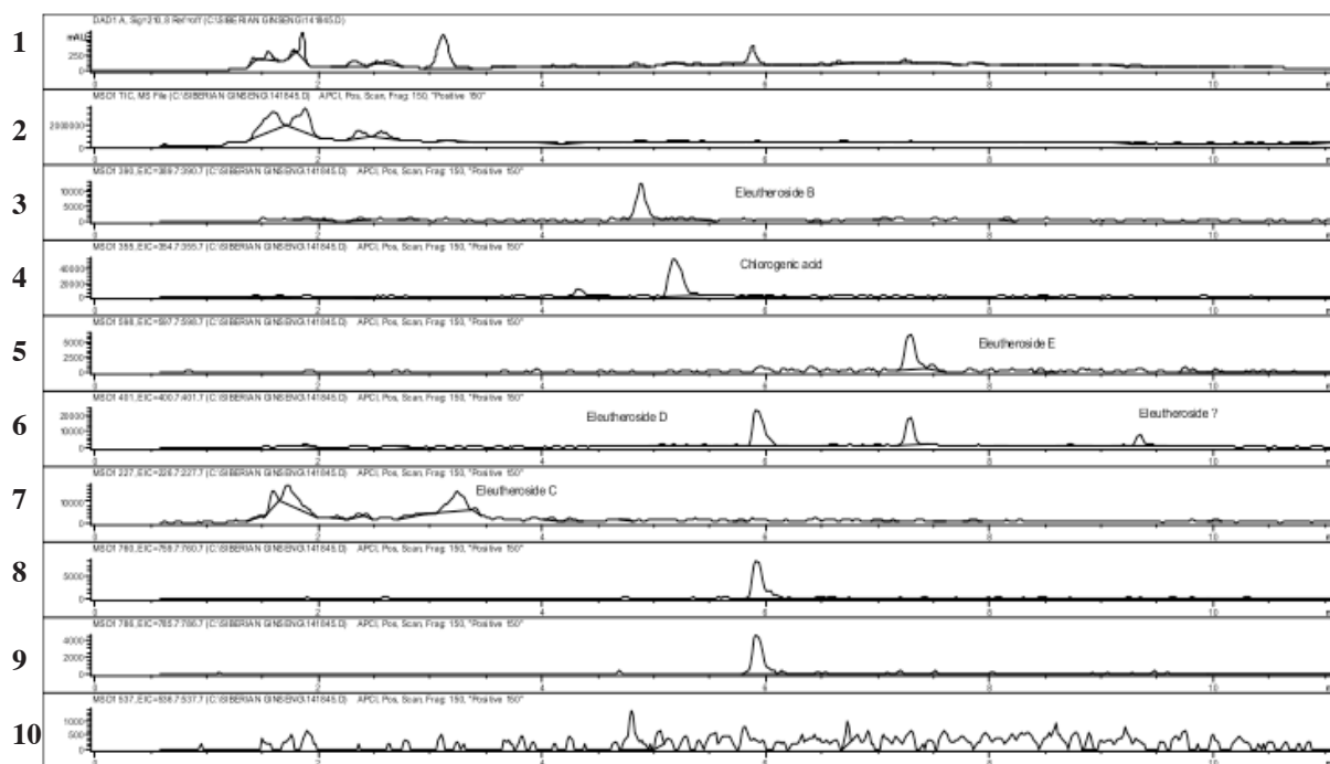
Figure 1. HPLC Trace of an E. senticosus (first 2 rows) as Performed by Southern Cross University Showing Eleutherodis B and E, and Chlorogenic Acid Detected. Individual phytochemicals (Eleutherodis B and E, and Chlorogenic acid) references shown in rows 3-10
