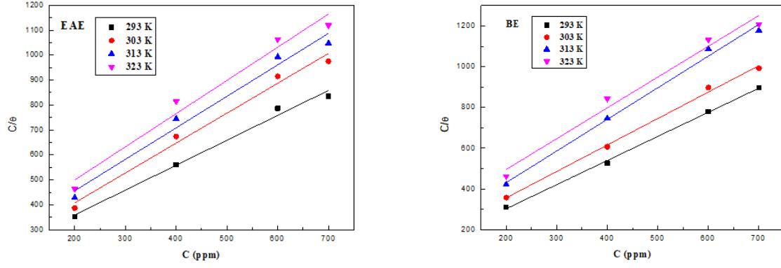
Figure 11: The Langmuir adsorption isotherm of HME, MDE, EAE, and BE on CS in a solution of 1M HCl at different temperatures.
