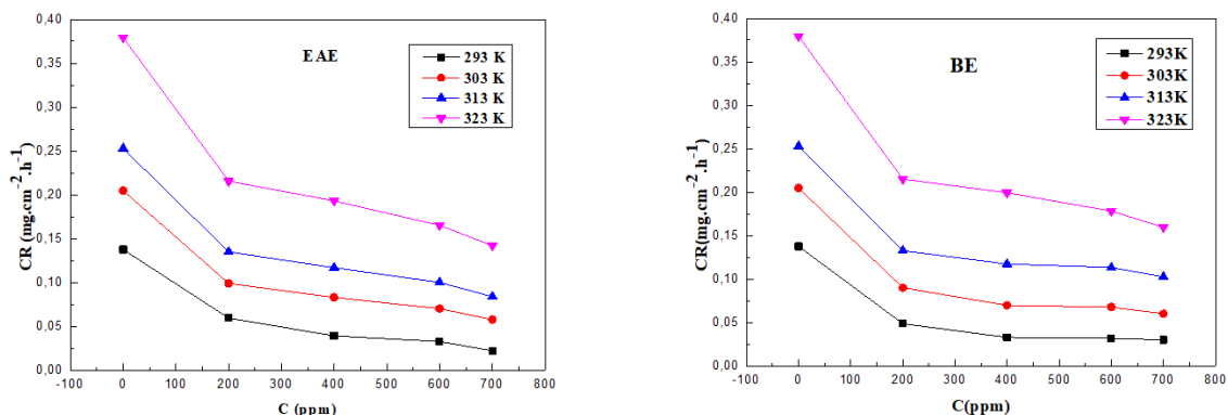
Figure 9: Variation of the corrosion rate as a function of various concentrations of HME, MDE, EAE, and BE in a 1M HCl solution at different temperatures.
