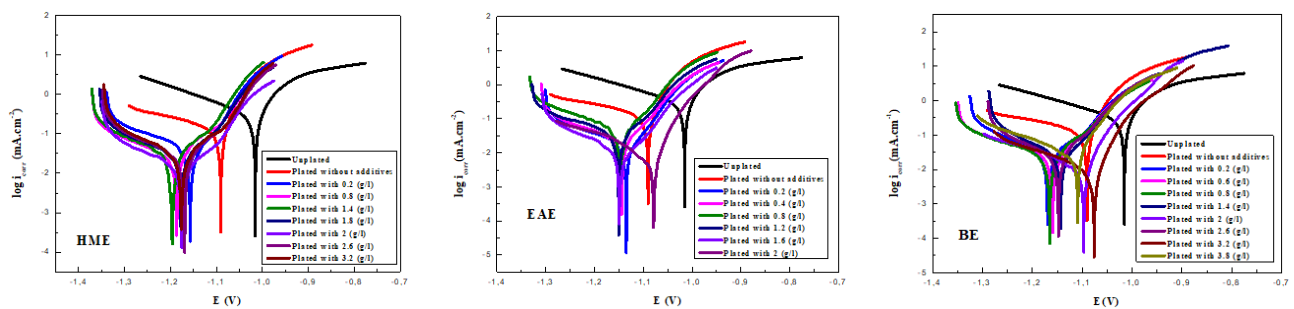
Figure 1: Potentiodynamic polarization curves for unplated and zinc-plated substrates without and with different concentrations of additives.
