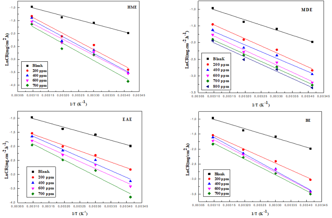
Figure 13: Arrhenius plots of \text{LnCR} versus \frac{1}{T} for CS corrosion in 1M HCl of HME, MDE, EAE, and BE.
