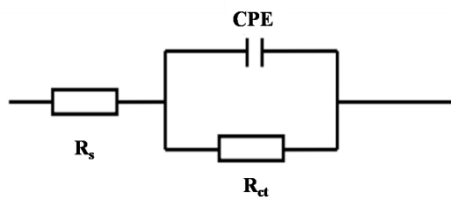
Figure 8: Equivalent circuit used to fit the capacitive loop.
