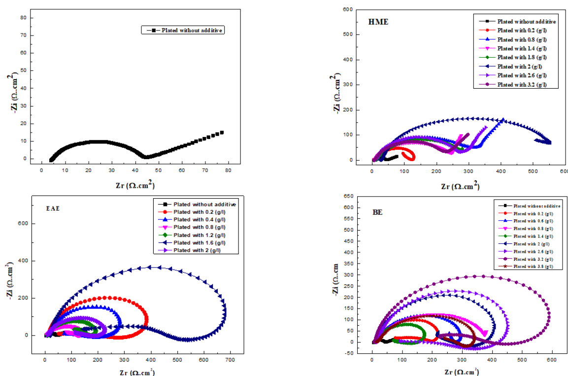
Figure 2: Electrochemical impedance plots of coated steels without and with the addition of different concentrations of additives.
