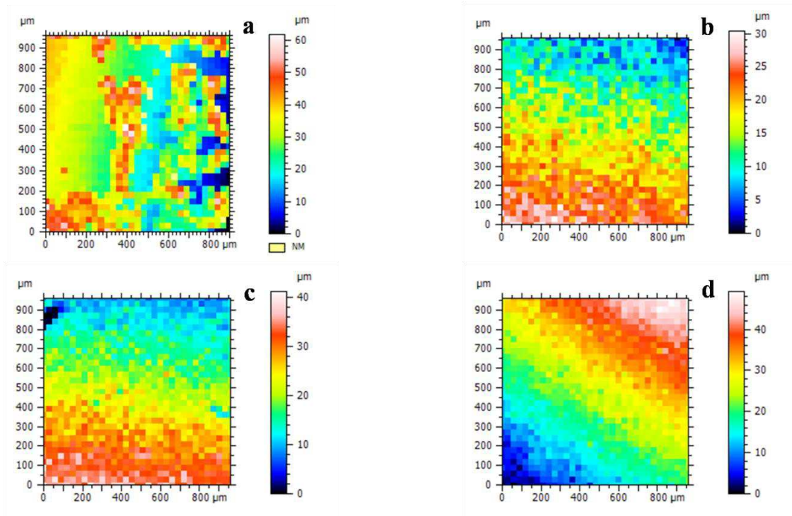
Figure 5: Profilometer 2D images of plated MS a) without extract addition, b) in the presence of 1.8 g/l of HME, c) in the presence of 0.2 g/l of EAE, and d) in the presence of 0.6 g/l of BE.
