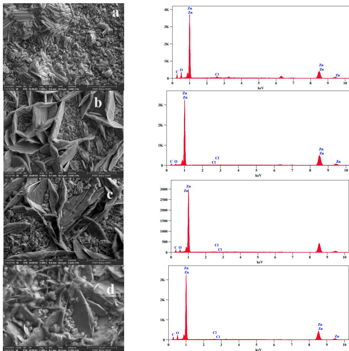
Figure 3: SEM/EDS images of: MS surface-plated a) without additive; b) in the presence of 1.8 g/l of HME; c) 0.2 g/l of EAE; and d) 0.6 g/l of BE.
