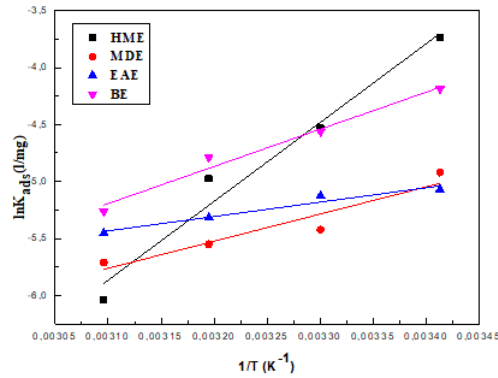
Figure 12: Variation of \ln K_{ads} as a function of the inverse of the temperature.
