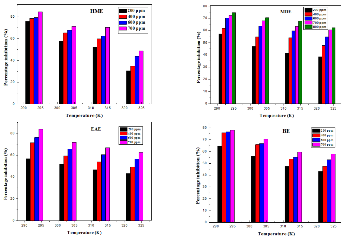
Figure 10: Temperature and concentration effects on HME, MDE, EAE, and BE inhibition efficiency in a 1M HCl solution.
