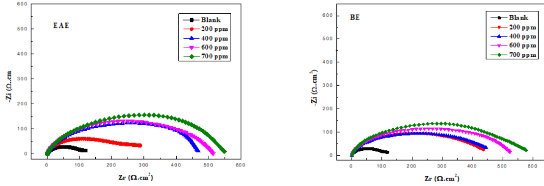
Figure 7: Nyquist diagrams for the CS in 1M HCl solution in the absence and presence of HME, MDE, EAE, and BE at various concentrations.
