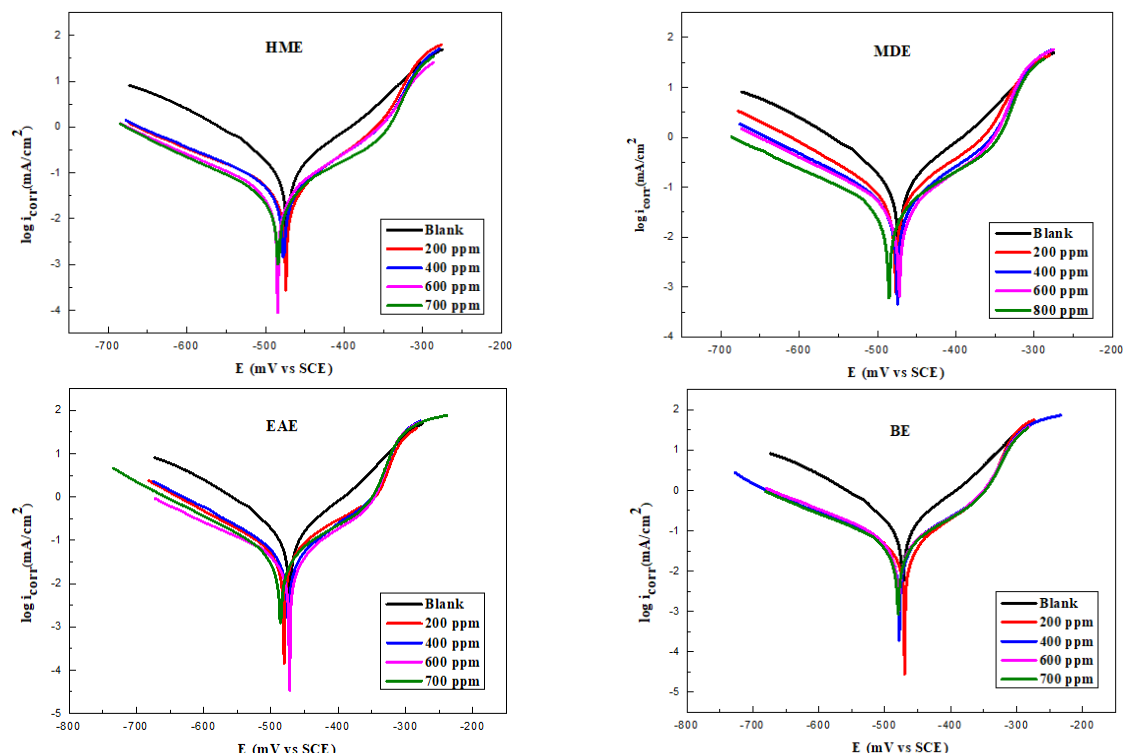
Figure 6: Potentiodynamic polarization curves of CS in 1M HCl without and with various amounts of HME, MDE, EAE, and BE.
