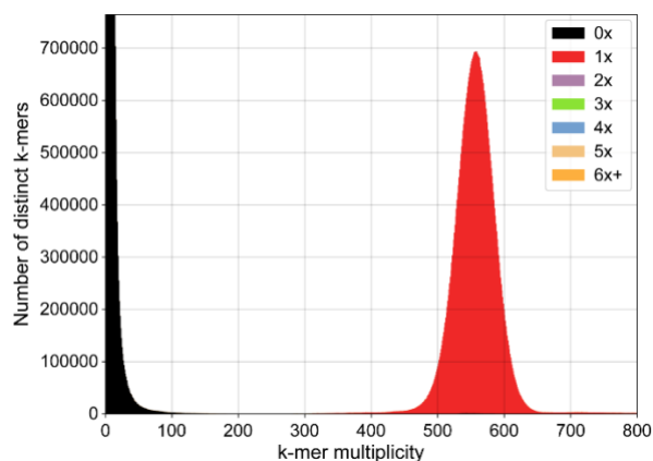
Figure 4 - The Coccomyxa viridis SAG 216-4 nuclear genome is haploid. The KAT spectra-cn plot depicts the 27-mer multiplicity of the PacBio HiFi reads against the nuclear genome assembly. Black areas under the peaks represent k-mers present in the reads but absent from the assembly, colored peaks indicate k-mers that are present once to multiple times in the assembly. The single red peak in the KAT spectra-cn plot suggests that Coccomyxa viridis has a haploid genome, while the black peak at low multiplicity shows that the assembly is highly complete and that all reads are represented in the assembly.
