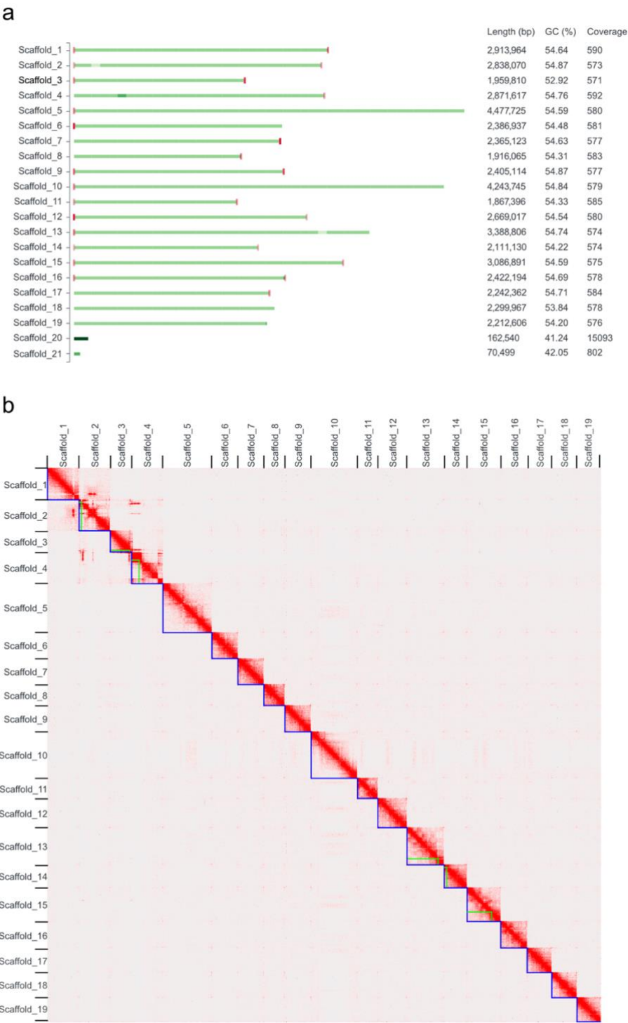
Figure 1 - Genome assembly of Coccomyxa viridis SAG 216-4. (a) An overview of the C. viridis genome assembly depicts chromosome-scale scaffolds. Green bars indicate scaffold sizes and red bars represent telomeres. Variations in color intensities correlate with read coverage. Read coverage per scaffold is determined by mapping PacBio HiFi reads onto the assembly. Scaffolds 20 and 21 were identified as chloroplast and mitochondrial genomes based on size and low GC contents, and BLAST analyses. (b) Hi-C contact map showing interaction frequencies between regions in the nuclear genome of Coccomyxa viridis . Scaffolds are framed by blue lines while contigs within scaffolds are depicted in green.
