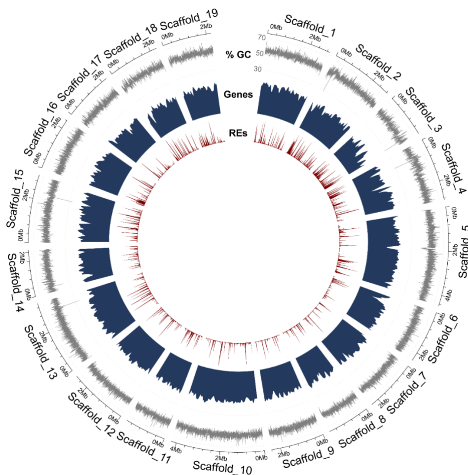
Figure 5 - Circos plot summarizing the nuclear genome annotation of Coccomyxa viridis SAG 216-4. From outside to inside the tracks display: GC content (over 1-kb windows), gene density (blue) and repetitive element density (red).
