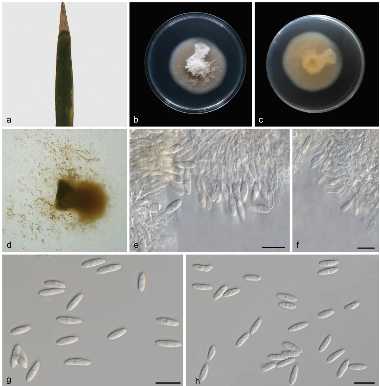
Figure 3. Microdochium baishamenense (CGMCC 3.28625, ex-holotype culture). a. A leaf of Phragmites australis ; b, c. Colonies on PDA from above and below after 7 days; d. Colony overview; e, f. Conidiogenous cells and conidia; g, h. Conidia. Scale bars: 10 µm ( e–h ).
