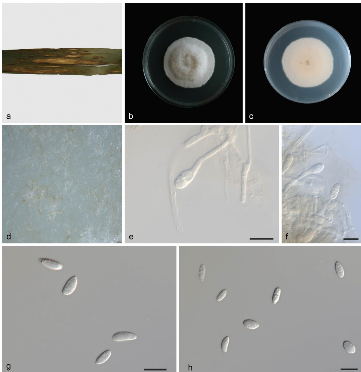
Figure 2. Microdochium australiana (CGMCC 3.28622, ex-holotype culture). a. A leaf of Phragmites australis ; b, c. Colonies on PDA from above and below after 7 days; d. Colony overview; e, f. Conidiogenous cells and conidia; g, h. Conidia. Scale bars: 10 µm ( e–h ).
