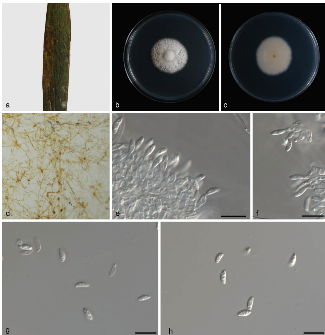
Figure 4. Microdochium bambusina (CGMCC 3.28623, ex-holotype culture). a. A leaf of Bambusaceae sp.; b, c. Surface and reverse sides of colony after 7 days on PDA; d. Colony overview with conidiomata; e, f. Conidiogenous cells with conidia; g, h. Conidia. Scale bars: 10 \mu\text{m} ( e–h ).
