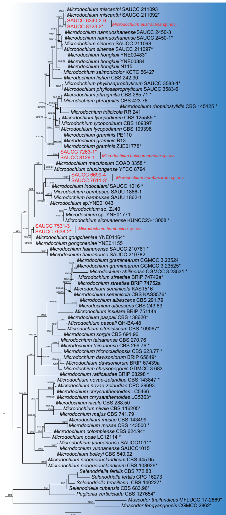
Figure 1. Maximum likelihood inference tree based on a combined dataset of analyzed ITS, LSU, rpb2 , and tub2 sequences. The Bayesian inference posterior probability (left, BIPP \geq 0.90 ) and the maximum likelihood bootstrap value (right, MLBV \geq 75\% ) are shown as BIPP/MLBV above the nodes. Those marked "*" in the tree are represented as ex-type or ex-epitype strains. Strains isolated in this study are indicated in red. The scale bar at the bottom indicates 0.07 substitutions per site. To enhance the visual appeal of the evolutionary tree layout, certain branches are shortened by two diagonal lines ("/") with the number of times.
