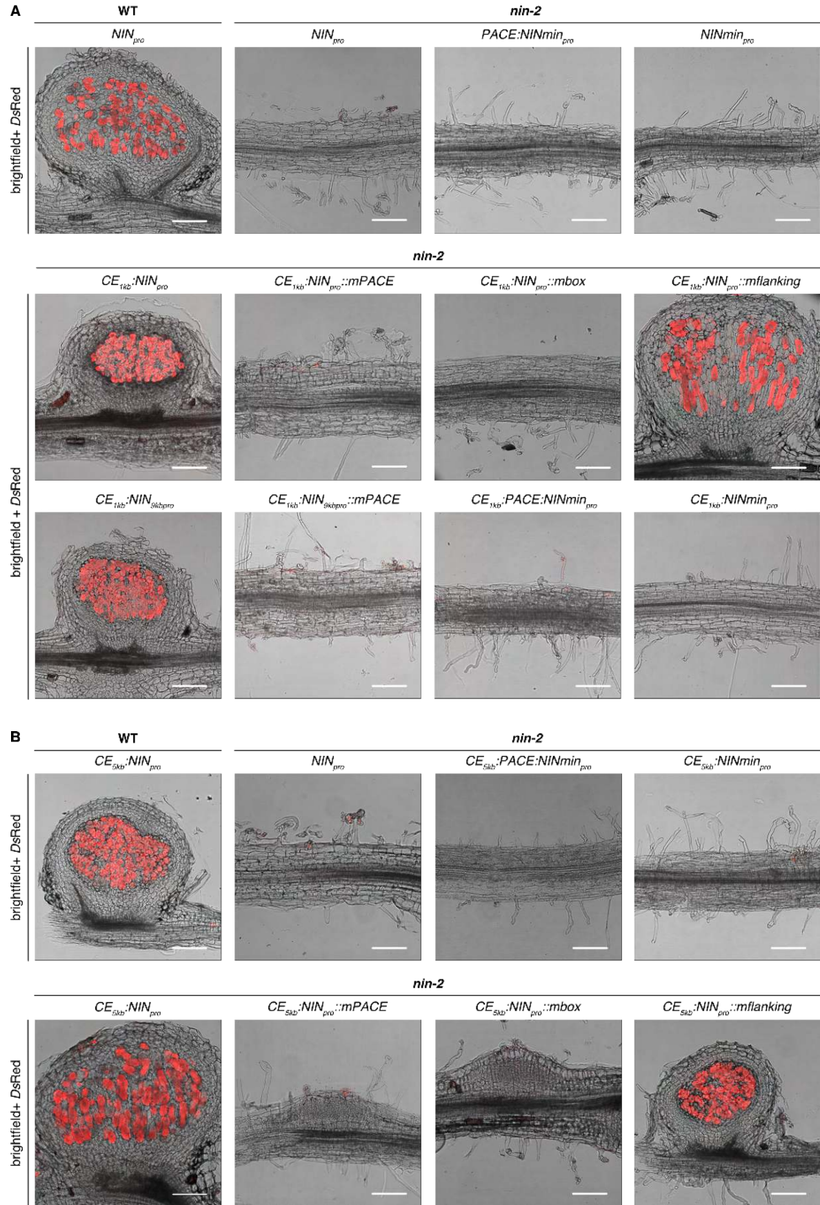
Figure 3 – figure supplement 5 | The CYC-box and flanking sequences of PACE are required for the complete restoration of the bacterial infection process but are dispensable for the nodule organogenesis process in the L. japonicus nin-2 mutant. Pictures of nodule sections or roots from L. japonicus nin-2 roots 21 dpi with M. loti DsRed from the same experiments depicted in Figure 3 – figure supplement 2 (A) and Figure 3 – figure supplement 4 (B) . Nodule sections from L. japonicus WT roots transformed with NIN pro :NIN and CE 5kb :NIN pro :NIN were included for comparison. Note that when the cytokinin element-containing region of 1 kb was fused to NIN pro nodule organogenesis was abolished by mutation of PACE or only the CYC-box in PACE and that these mutations did not abolish organogenesis when the cytokinin element-containing region of 5 kb was fused to NIN pro . Bars, 100 \mu m.
