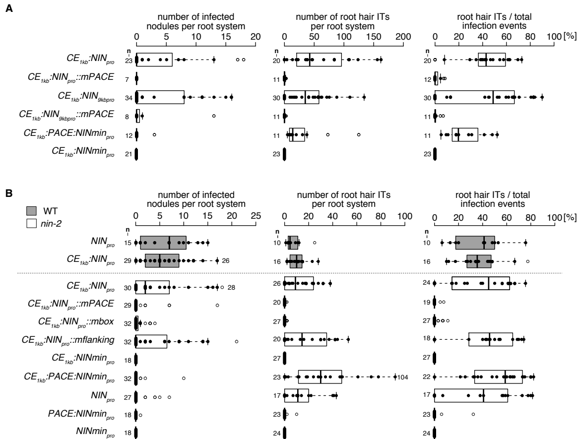
Figure 3 – figure supplement 3 | The CYC-box and flanking sequences of PACE are required for the complete restoration of the bacterial infection process in the L. japonicus nin-2 mutant. Roots were from a subset of plants from the same experiment depicted in Figure 3 – figure supplement 2 but analysed 35 dpi with M. loti DsRed. (A - B) Boxplots displaying the number of root hair ITs or infected nodules and the percentage of root hair ITs among total infection events (sum of bacterial entrapments and ITs). Each dot represents one transgenic nin-2 root system or root piece. L. japonicus WT roots transformed with NIN_{pro}::NIN or CE_{1kb}::NIN_{pro}::NIN were included as controls. Note that the results follow the same trend as those obtained 21 dpi with M. loti DsRed ( Figure 3 – figure supplement 2 ). n : number of transgenic root systems or root pieces analysed. Numbers above the boxplots: the value of individual data points outside of the plotting area.
