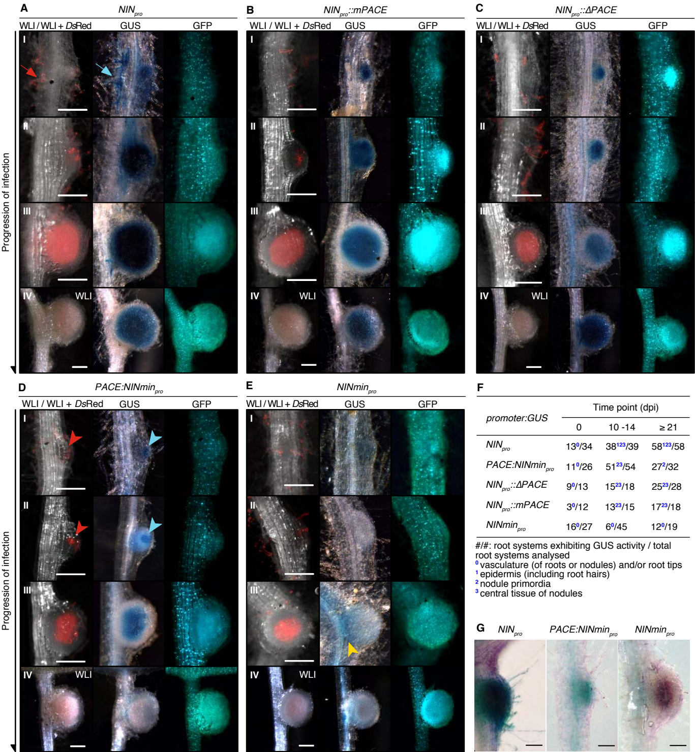
Figure 2 – figure supplement 1 | Spatio-temporal GUS expression driven by PACE and the NIN promoter in L. japonicus roots during the bacterial infection process. L. japonicus wild-type hairy roots were transformed with T-DNAs carrying a Ubq10 pro ::NLS-GFP transformation marker together with a GUS reporter gene driven by either of the indicated promoters: (A) the 3 kb LjNIN promoter ( NIN pro ); the LjNIN promoter with PACE (B) mutated ( LjNIN pro ::mPACE ) or (C) deleted ( NIN pro ::ΔPACE ); (D) PACE fused to the LjNIN minimal promoter ( PACE:NINmin pro ) or (E) the LjNIN minimal promoter ( NINmin pro ). The progression of bacterial infection was determined by the DsRed signal 10 - 14 days post inoculation (dpi) with M. loti DsRed . Nodules undergoing different stages of infection (panels I to IV) were stained with X-Gluc to reveal the GUS expression pattern. Note the overlapping bacterial invasion zone and PACE:NINmin pro ::GUS expression in early infection stages (red and blue arrowheads in (D)) as well as the differences between PACE:NINmin pro ::GUS and the much broader NIN pro ::GUS expression at that stage (red and blue arrows in (A)). Red arrow and arrowheads: M. loti DsRed . Blue arrow and arrowheads: GUS activity in root hairs bearing ITs and nodule primordia, respectively. The NINmin pro ::GUS fusion gave only rarely detectable signal, and if so in the vasculature (yellow arrowhead in (E)). Only pictures taken under white light illumination (WLI) are displayed for nodules in panel VI to reveal the pink colour of leghemoglobin, characteristic for mature and fully infected nodules. Note that PACE:NINmin pro ::GUS expression was absent at this stage, whereas the NIN pro ::GUS resulted in strong blue staining in the nodule regardless of the presence of PACE (compare panel IV in (D) and (A - C)). (F) Quantification of transgenic root systems exhibiting GUS expression in different cell types and tissues exemplarily displayed in (A - E). (G) PACE drove GUS reporter gene expression in the central tissue of primordia and nodules, but was not sufficient for expression in root hairs. Transgenic roots carrying promoter: GUS fusions same as in (A, D and E) were inoculated with M. loti lacZ and dual-stained with X-Gluc and Magenta-Gal. Purple: M. loti lacZ . Blue: GUS activity. Note the co-existence of blue and purple staining in root hairs on roots transformed by NIN pro ::GUS , but not that transformed by PACE:NINmin pro ::GUS . Bars, 250 μm.
