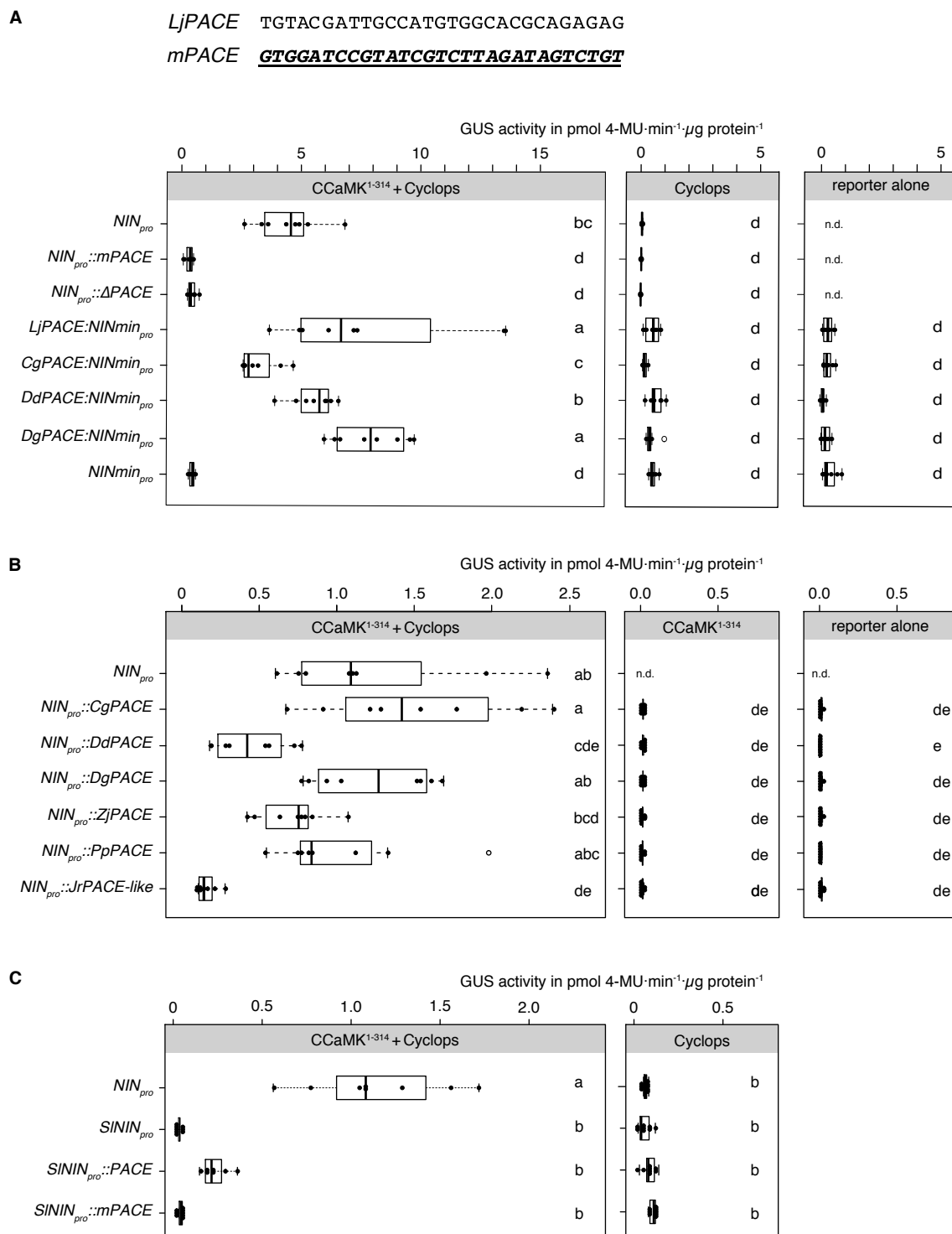
Figure 1 – figure supplement 6 | PACE sequence variants from species across the FaFaCuRo clade were able to functionally replace L. japonicus PACE in a LjNIN pro ::GUS reporter fusion. N. benthamiana leaf cells were transformed with T-DNAs carrying a GUS reporter gene driven by either of the indicated promoters: (A) the L. japonicus NIN promoter ( NIN pro ), the LjNIN promoter with PACE mutated or deleted ( NIN pro ::mPACE and NIN pro ::ΔPACE , respectively), or PACE sequence variants from the nodulating FaFaCuRo species fused to the LjNIN minimal promoter ( NINmin pro ); (B) chimeric promoters where LjPACE in the LjNIN promoter was replaced with either one of the PACE variants from species tested in (A) or from non-nodulating FaFaCuRo species including the Juglans regia PACE -like motif ( JrPACE-like ); (C) the S. lycopersicum NIN promoter ( SININ pro ), the SININ promoter with LjPACE ( SININ pro ::PACE ) or mPACE ( SININ pro ::mPACE ) inserted. For species abbreviations see Figure 1 – figure supplement 5A . Note in (A) that the deletion or mutation of PACE in LjNIN promoter resulted in a drastic reduction in reporter gene expression and in (C) insertion of LjPACE but not mPACE into the S. lycopersicum promoter confers transactivation by CCaMK 1-314 /Cyclops. The applied statistical method was ANOVA with post hoc Tukey: (A) F_{20,144} = 51.38 , p < 2 \times 10^{-16} ; (B), F_{18,186} = 149.1 , p < 2 \times 10^{-16} ; (C) F_{7,62} = 30.5 , p = 7.02 \times 10^{-7} . Different small letters indicate significant difference. n.d., not determined.
