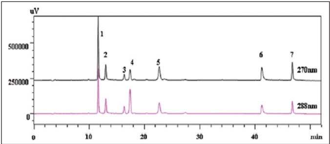
Figure 2. Chromatogram of marker compound according to Li et al. [11].
