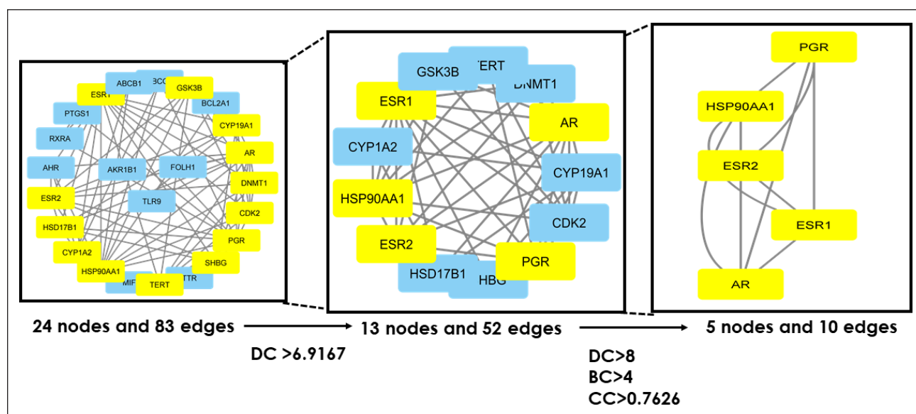
Figure 4. The inter-protein interaction analysis was conducted using the CytoNCA plug-in in two screening steps. In the final results, five core targets—PGR, HSP90AA1, ESR2, ESR1, and AR—were identified based on three centrality parameters: DC, BC, and closeness centrality (CC).
