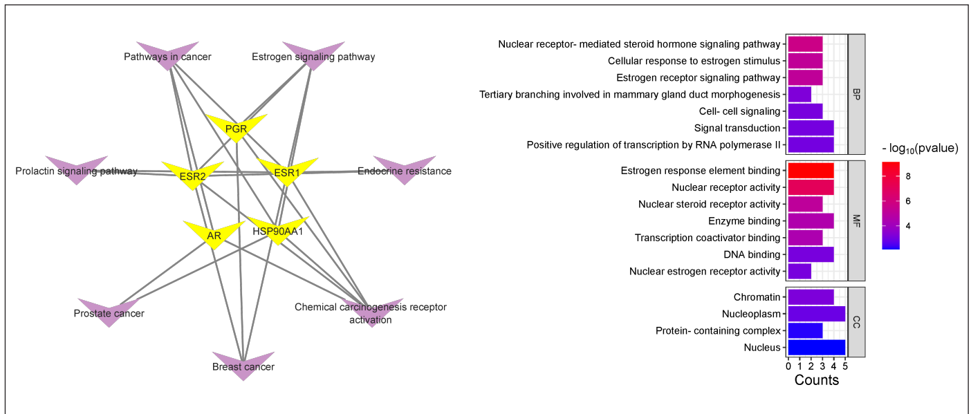
Figure 5. KEGG pathway analysis of target genes shortlist by top seven representative pathways according to gene (a), GO search results of potential targets of amentoflavone and 2,3-Dihydro-3,3-biapiogenin on cervical cancer, including BP, cellular components and MFs (b).
