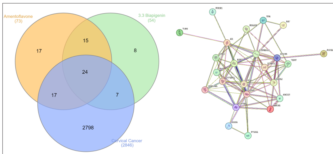
Figure 3. PPI network using STRING.
