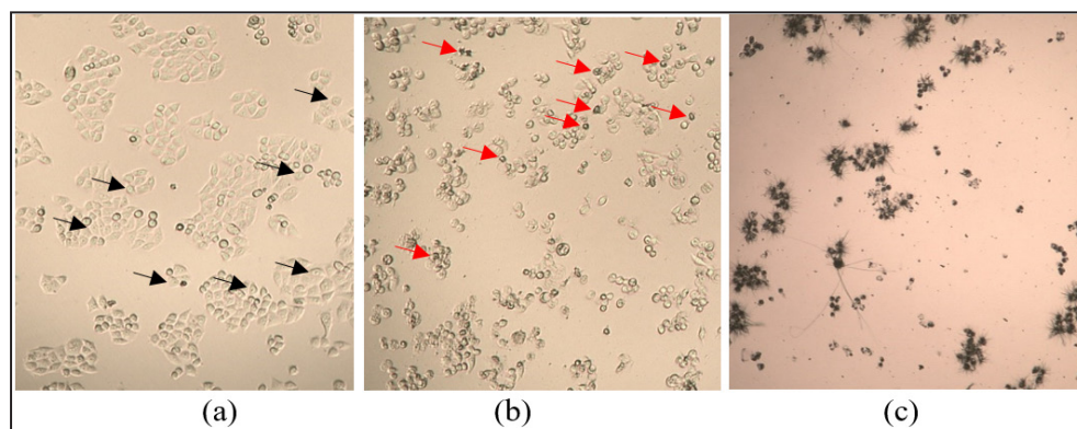
Figure 9. Morphological changes of HeLa cells on treatment with EESD (a) Before treatment, (b) After treatment, (c) After MTT reagent addition. (—) live cells; (—) dead cells.
