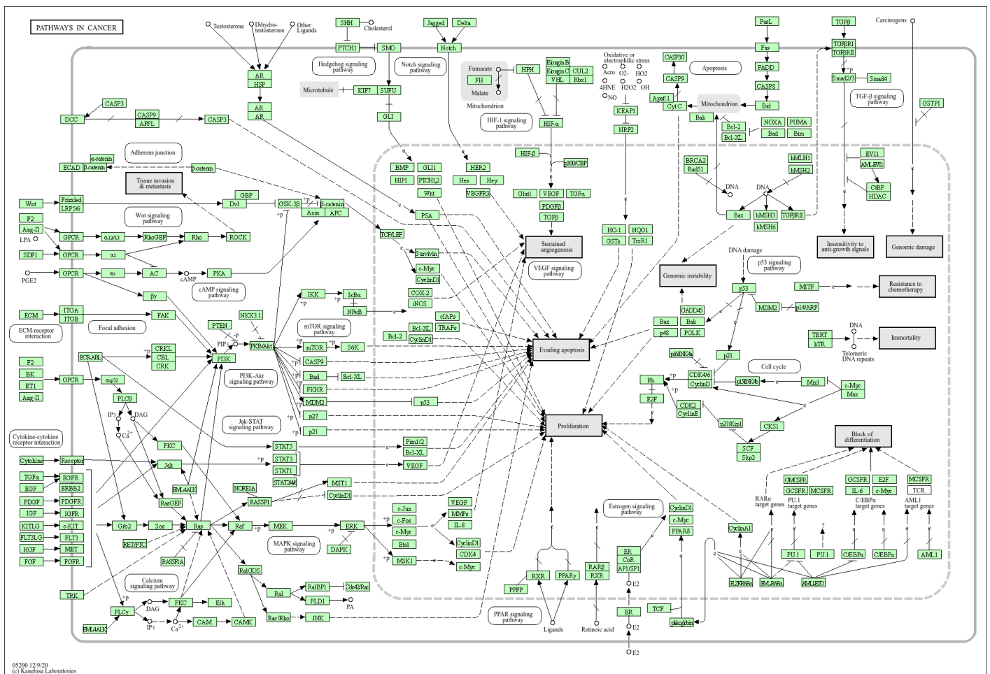
Figure 6. Major protein target signaling pathway in cancer [15,20].
