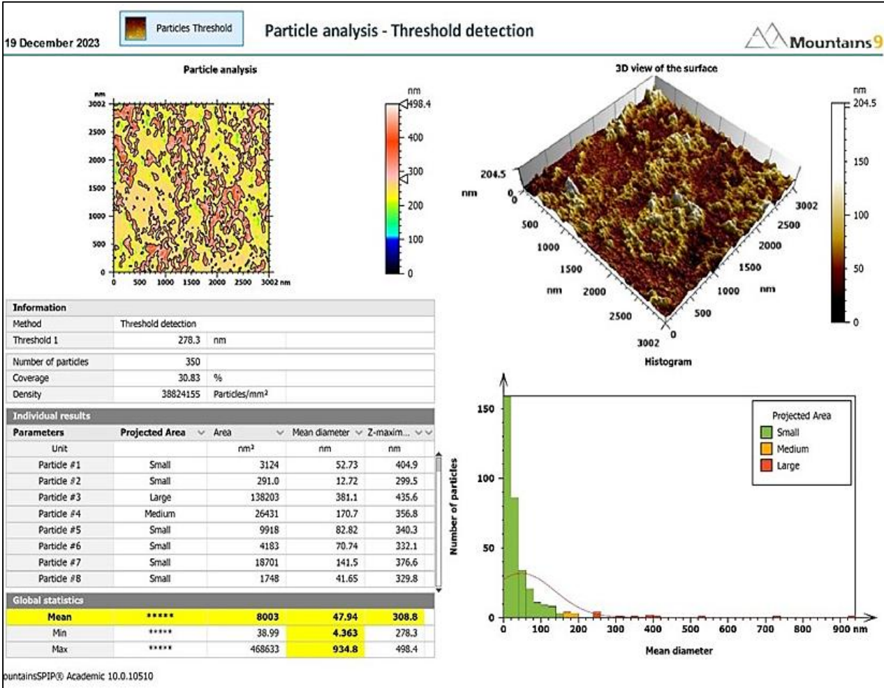
Fig. 4. AFM surface and Histogram for grain accumulation.
