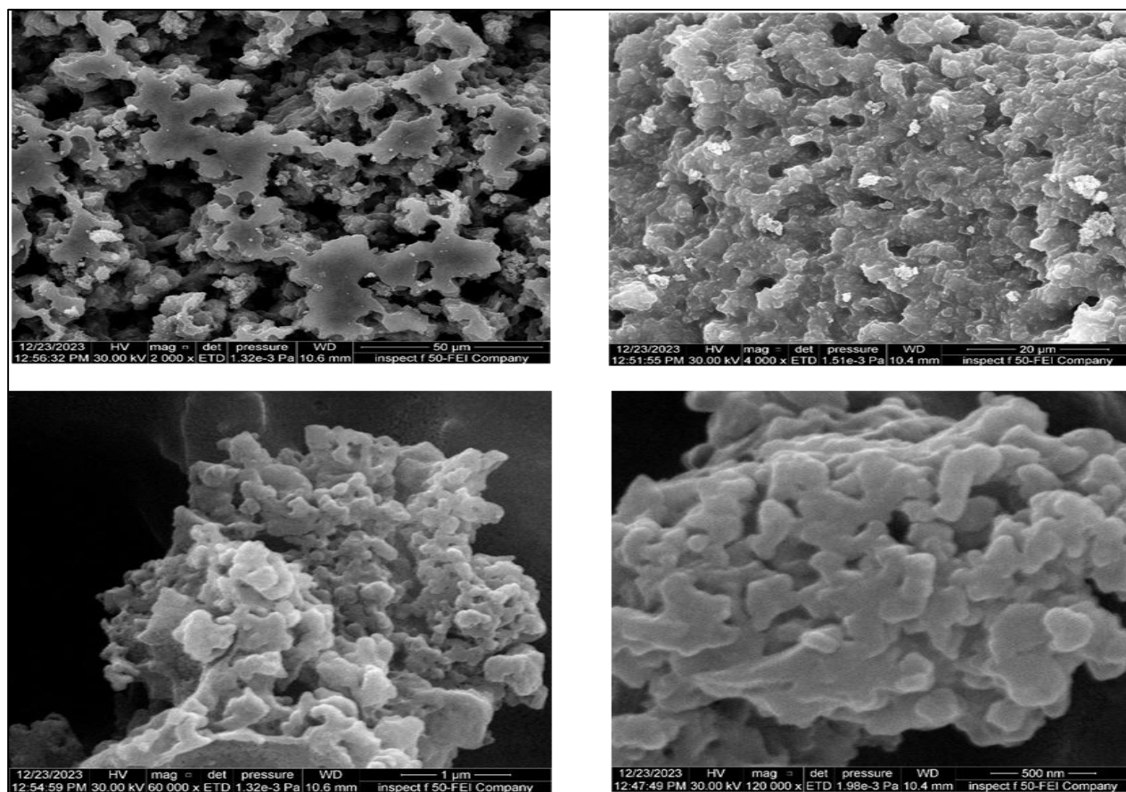
Fig. 2. FE-SEM analysis of \text{Fe}_2\text{O}_3 .
