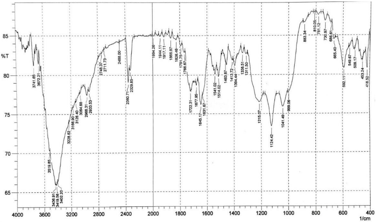
Fig. 5. FTIR spectroscopy Fe 2 O 3 Nanoparticles.
