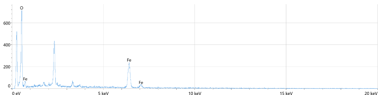
Fig. 3. EDX analysis of \text{Fe}_2\text{O}_3 nanoparticles.
