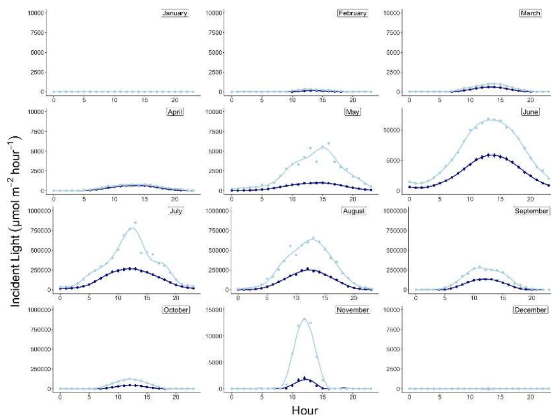
FIGURE 3 Daily average (navy) and maximum (light blue) incident light profiles by month at 15m depth in Arctic Bay, Nunavut, Canada across the experimental period. Note differences in y-axis scales.
