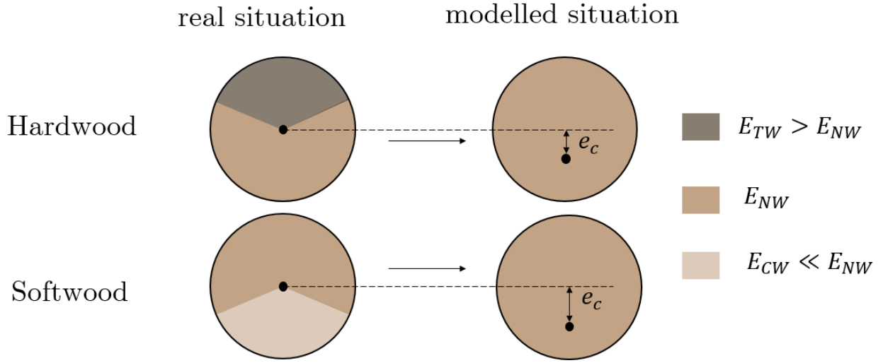
Figure 11: How the hypothesis of a uniform wood stiffness impacts the initial position of the pith. e_c : pith offset equivalent to a centered pith with heterogenous wood properties; E_{TW} , E_{NW} , E_{CW} : Longitudinal Young’s modulus of tension, normal, compression wood, respectively.
