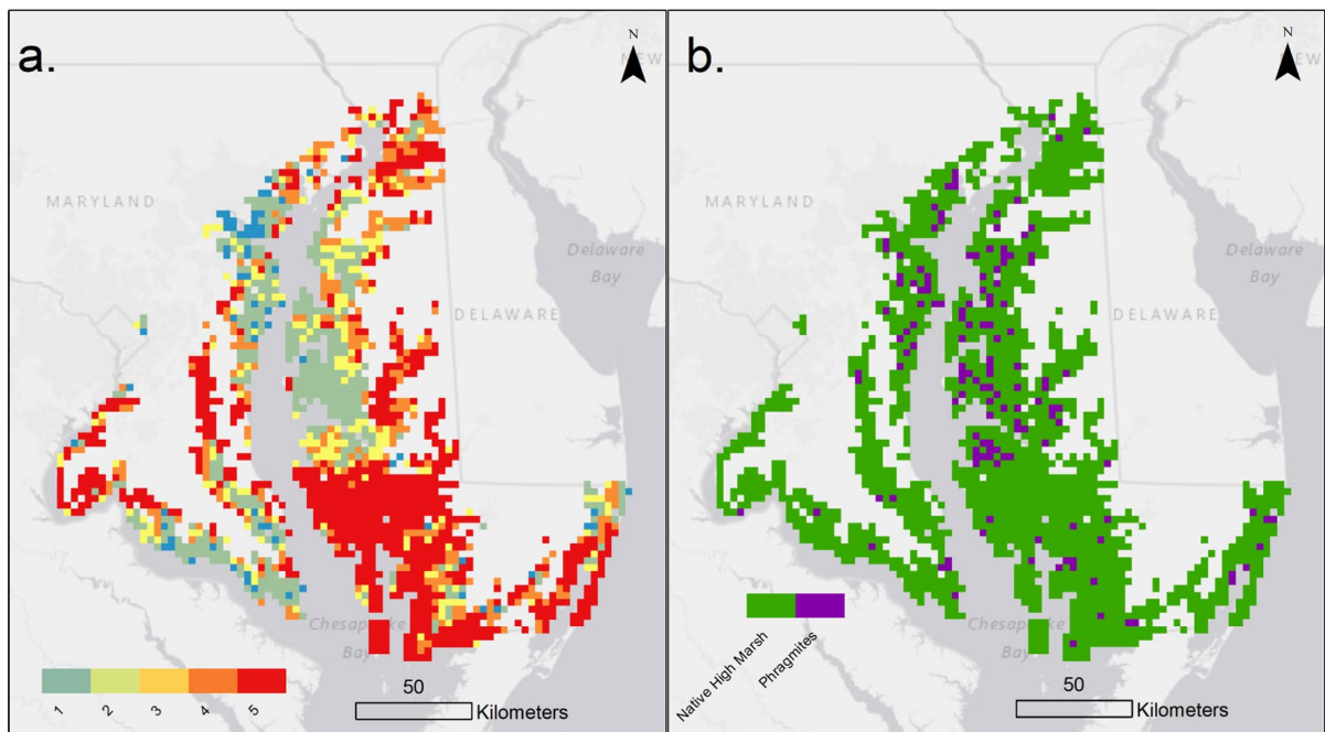
Fig. 3 Comparison of Wildlife Habitat and Biodiversity Index (panel a) and occurrence of Phragmites australis (panel b) in the Chesapeake Bay region
