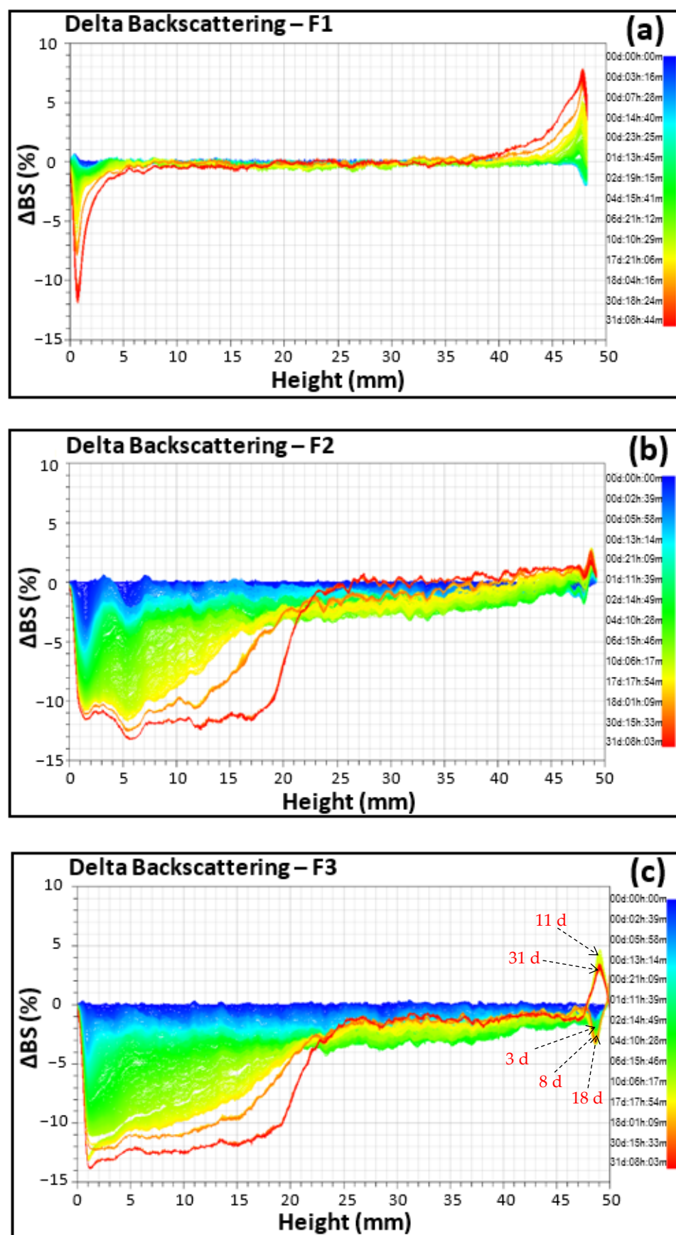
Figure 5. Delta backscattering signals of emulsions F1 (a), F2 (b) and F3 (c).
