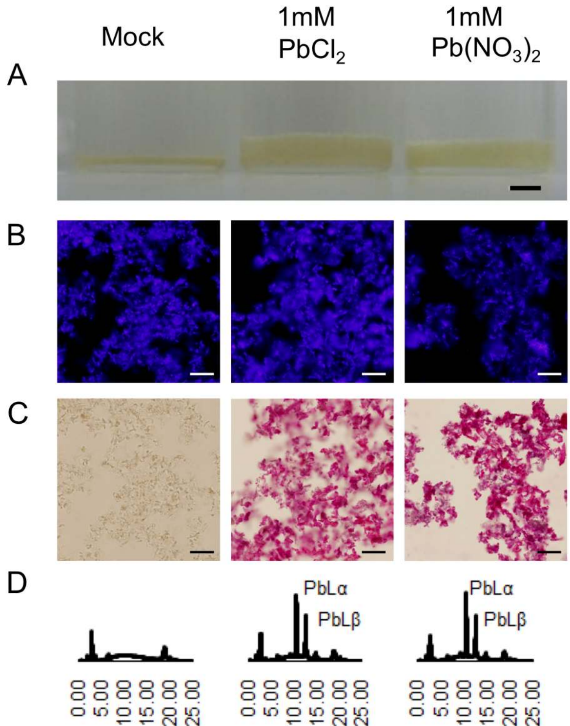
Fig 3. Adsorption of Pb to prepared a cell-wall fraction of F. hygrometrica . Aliquots of a cell-wall (CW) fraction were suspended in MQW (Mock), 1 mM \text{PbCl}_2 , or 1 mM \text{Pb}(\text{NO}_3)_2 . After washing with MQW, Pb was detected with rhodizonic acid staining and X-ray analysis. (A) Precipitated CW fractions in bottles after treatment. (B) Autofluorescence image of rhodizonic acid-stained CW fraction observed with Bio Imaging Navigator with a fluorescence filter (FSX100/U-MNUA2, OLYMPUS, Japan). (C) Observation with bright field mode. (D) Spectra of X-ray analysis with an X-ray analyzer. Background peaks in mock treatment are derived from rhodizonic acid. Scale bars, 3 mm in (A), 100 \mu\text{m} in (B) and (C).
