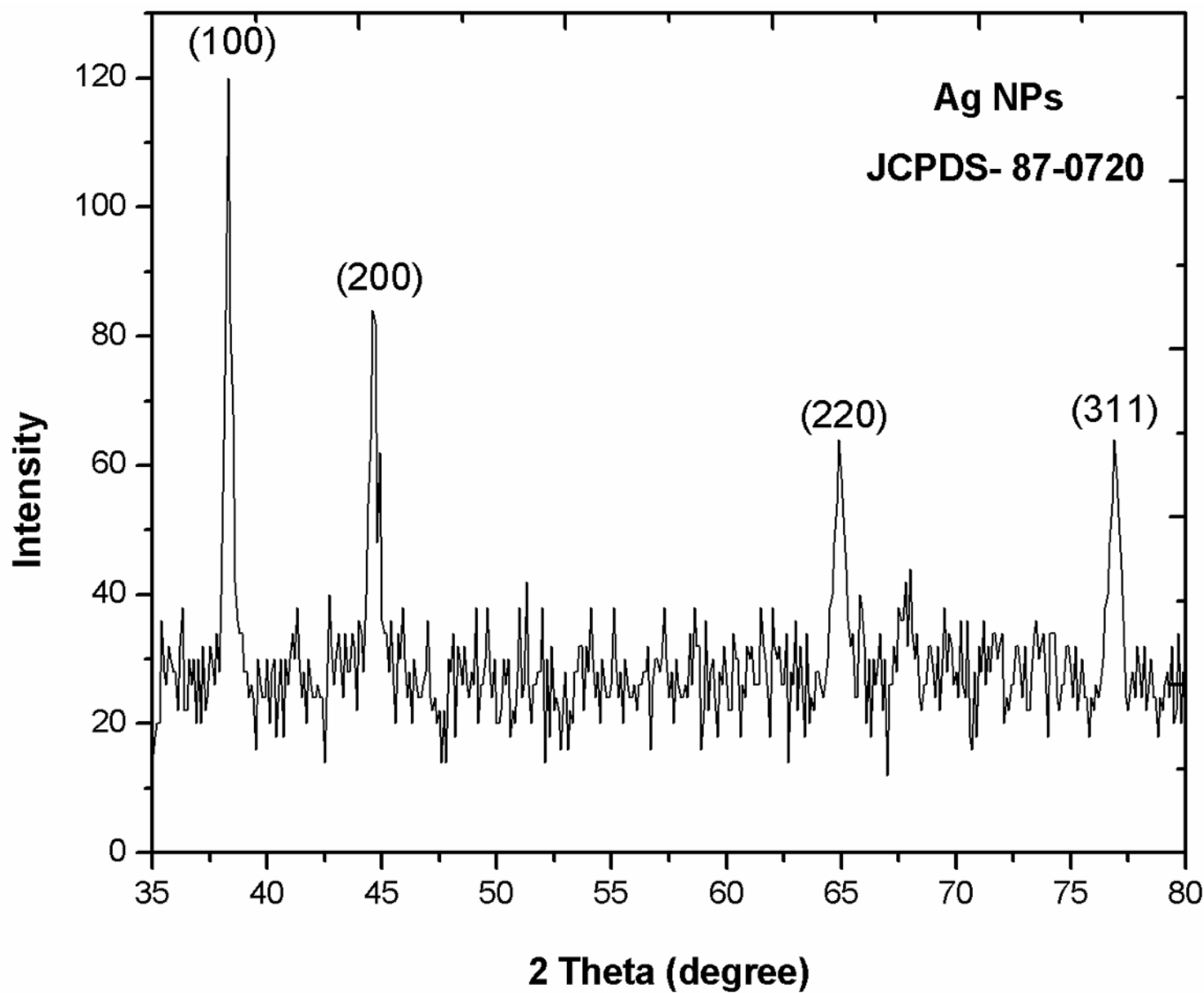
Figure 6 XRD analysis of Pa-AgNPs
