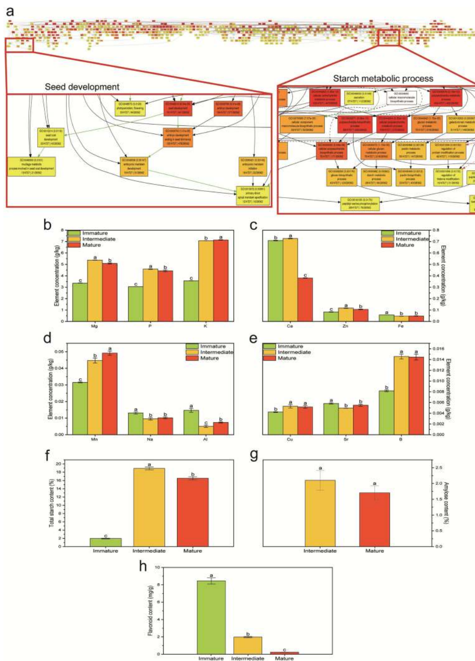
Fig. 5 GO functional annotation and physiological–biochemical changes during seed development in S. lanceolata . (a) GO functional annotation of S. lanceolata , with seed development and starch metabolism highlighted within the red box. (b–e) Changes in mineral element contents in seeds at different developmental stages. (f) Changes in total starch content in seeds at various developmental stages. (g) Changes in amylose content in seeds at different developmental stages. (h) Changes in flavonoid content in seeds at different developmental stages
