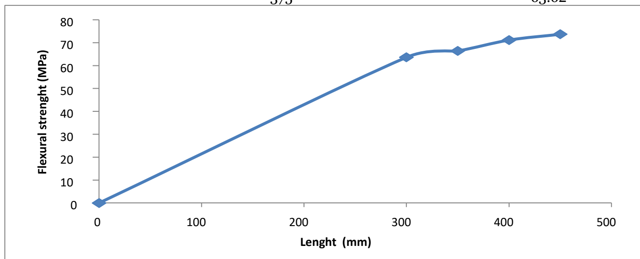
Figure 6: Flexural strength graph of composite bumper
