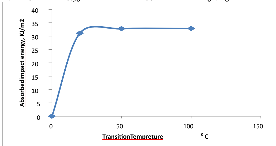
Fig. 3: Impact strength graph of composite bumper
