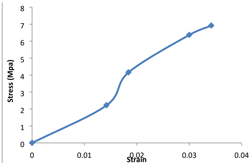
Figure 5: Compressive strength graph of composite bumper Flexural test of composite bumper.
