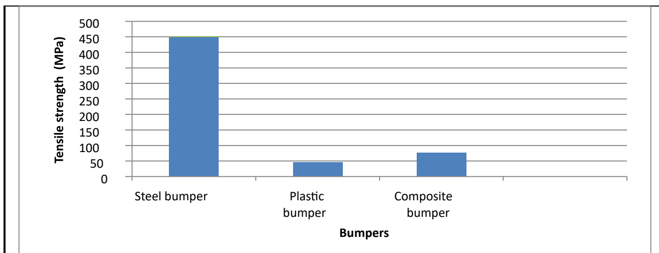
Figure 12. Tensile Strength Comparison of bumpers
