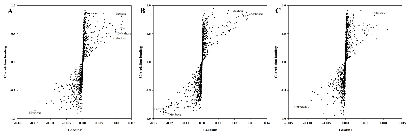
Fig. 3 S-plot based on orthogonal partial least squares-discriminant analysis using gas chromatography-mass spectrometry data (A) for comparative analysis of honeys collected from Janghang Wetland in March (positive direction) and April (negative direction), (B) for comparative analysis between honeys collected from Janghang Wetland (positive direction) and apiculture honeys (negative direction) and (C) for comparative analysis between higher Prunus and Salix ratio ( Prunus > Salix : positive direction; Prunus < Salix : negative direction) among honeys collected from Janghang Wetland. Only identified metabolites were given names among the metabolites considered meaningful. Metabolites deemed meaningful were not identified in (C).
