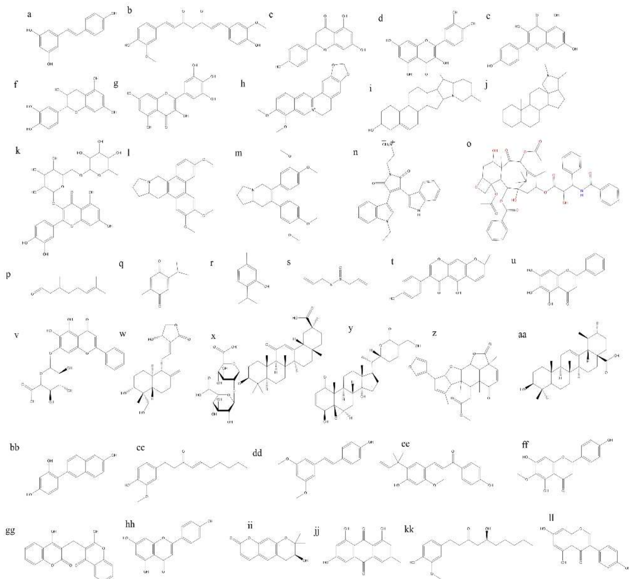
Figure 3. Chemical structures of some anticancer phytoconstituents. a: resveratrol; b: curcumin; c: naringnin; d: quercetin; e: kaepferol; f: epicatechin; g: myricetin; h: berberine; i: solaidine; j: conanine; k: rutine; l: antoline; m: tylophorine; n: BMA-155Cl; o: paclitaxel; p: citronellal; q: thymoquinone; r: thymol; s: allicin; t: alpinumisoflavone; u: baicalein; v: baicalin; w: andrographolide; x: glycyrrhizin; y: withaferin A; z: nimbolide; aa: ursolic acid; bb: resveratrol analogue HS-1793; cc: 6-shogaol; dd: pterostillben; ee: licochalcone A; ff: hispudilin; gg: dicoumarol; hh: apigenin; ii: decursinol; jj: emodin; kk: gingerol; ll: genistein
