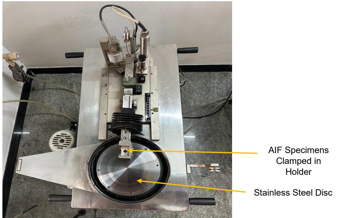
Figure 4: Pin-on-Disc Wear Testing Setup
