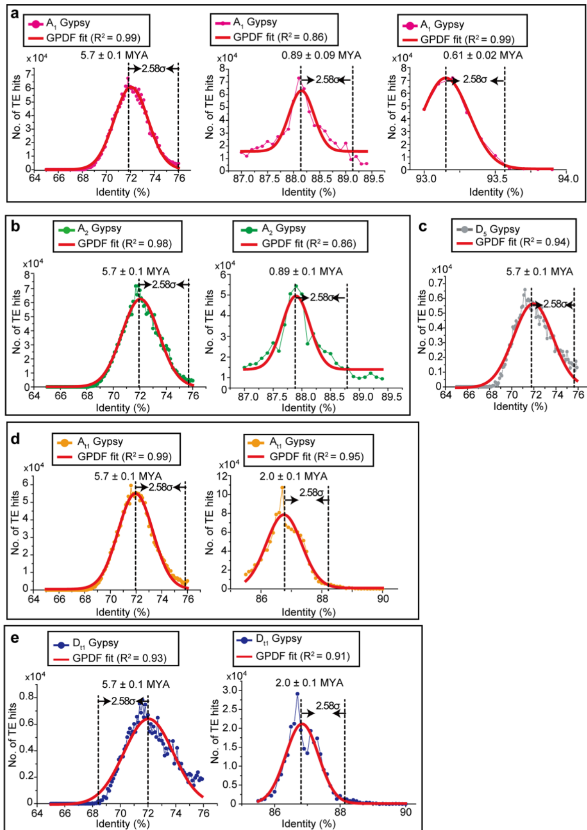
Extended Data Fig. 9 | The burst of LTR/Gypsy amplification fits a Gaussian distribution and allows time estimation of burst events. a–e , GPDM modeling data fit well with the actual TE bursts found in A_1 with R^2 from 0.86–0.99 ( a ), A_2 with R^2 from 0.86–0.98 ( b ), D_5 with R^2=0.94 ( c ), A_{t1} with R^2 from 0.95–0.99 ( d ) and D_{t1} with R^2 from 0.91–0.93 ( e ). The estimated time of the LTR/Gypsy burst event associated with each genome or subgenome is shown in the graphs. The peak width was defined as 2.58\sigma that covers >99.5% of the nucleotide substitution events in TEs.
