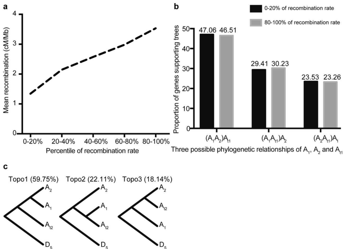
Extended Data Fig. 6 | Phylogenetic relationship among A_1 , A_2 and A-subgenome. a , Distribution of mean recombination rates in protein-coding genes with available recombination rates ( n = 240 genes). b , Proportion of genes with 0-20% and 80-100% of recombination rates supporting the three trees. c , Summary of phylogenetic analysis with the AU test in 10 kb windows among A_1 , A_2 , A_{t2} , D_5 .
