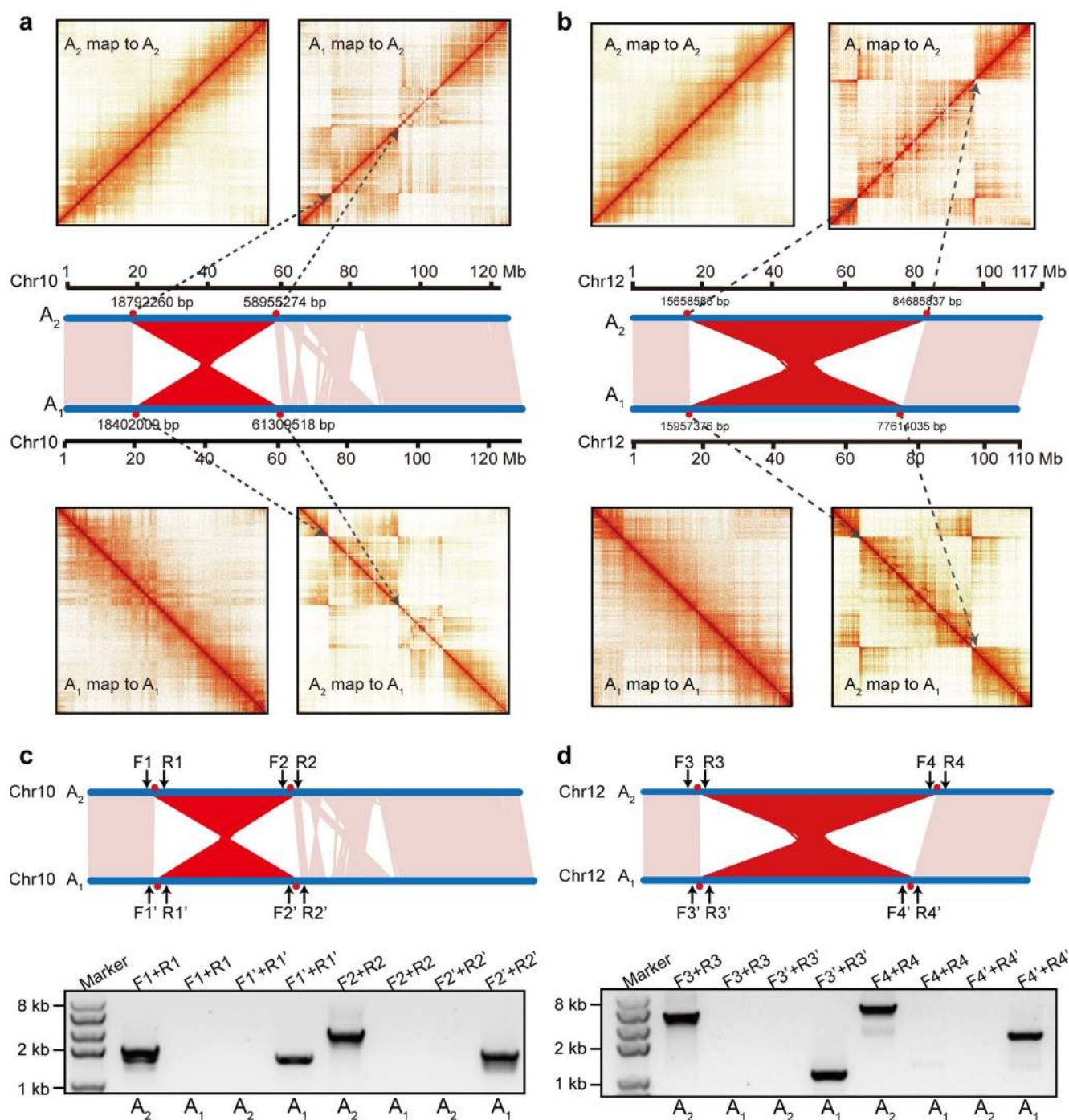
Extended Data Fig. 5 | Hi-C data and PCR amplification validate the border of two large inversions in chromosomes 10 and 12 between A_1 and A_2 genomes. a, b Identification of the ~42.9-Mb large inversion in chromosome 10 ( a ) and ~61.6-Mb large inversion in chromosome 12 ( b ) by Hi-C data. The upper heatmap shows a chromatin interaction matrix that maps Hi-C data from A_2 against the A_2 -genome ( A_2 map to A_2 ), and maps Hi-C data from A_1 against the A_2 -genome ( A_1 map to A_2 ). The middle panel shows a diagram of the inversion region with the four red dots representing the inversion borders. The lower heatmap shows a chromatin interaction matrix that maps Hi-C data from A_1 against the A_1 -genome ( A_1 map to A_1 ) and maps Hi-C data from A_2 against the A_1 -genome ( A_2 map to A_1 ). c, d Validation of inversion borders in chromosomes 10 ( c ) and 12 ( d ) by PCR amplification. The forward and reverse primer sequences are shown in Supplementary Table 16. The unprocessed gel for the cropped images are presented in source data.
