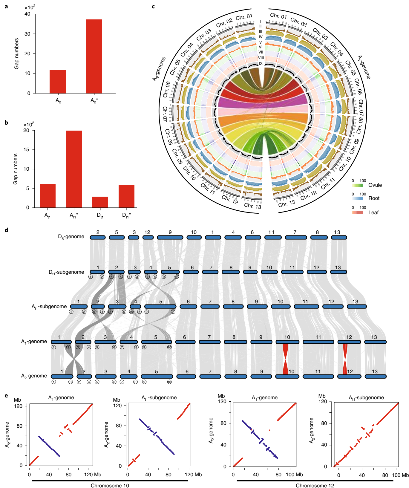
Fig. 1 | Distribution of genomic components of A_1 and A_2 across chromosomes and chromosomal variant events within the Gossypium lineage. a,b , Statistics of gap numbers in the assembly of A_2 - ( a ) and (AD)_{11} - ( b ) genomes. A_2^* , previously released A_2 -genome 18 ; A_{11}^* and D_{11}^* represent the A_{11} - and D_{11} -subgenome, respectively, of recently released (AD)_{11} -genome 21 . c , Multi-dimensional display of genomic components of A_1 - and A_2 -genomes. The density was calculated per 1Mb. I, the 13 chromosomes; II, gene density; III–V, coverage by TE, Gypsy and Copia, respectively; VI–VIII, transcriptional state in the ovule at 10 DPA and in root and leaf tissue, respectively. Transcript levels were estimated based on the average depth of mapped RNA reads in nonoverlapping 1-Mb windows. IX, GC content. d , Characterization of genomic variations in Gossypium . Genic synteny blocks are connected by gray lines. Reciprocal translocations and two large inversions are highlighted by dark gray and red links, respectively. e , Synteny maps using whole-genome alignments show that the inversion in chromosome 10 exists in either A_1 or A_{11} , whereas the one in chromosome 12 is found only in A_1 . Genomic homologous blocks \geq 20 kb are drawn in the plots. Chr, chromosome.
