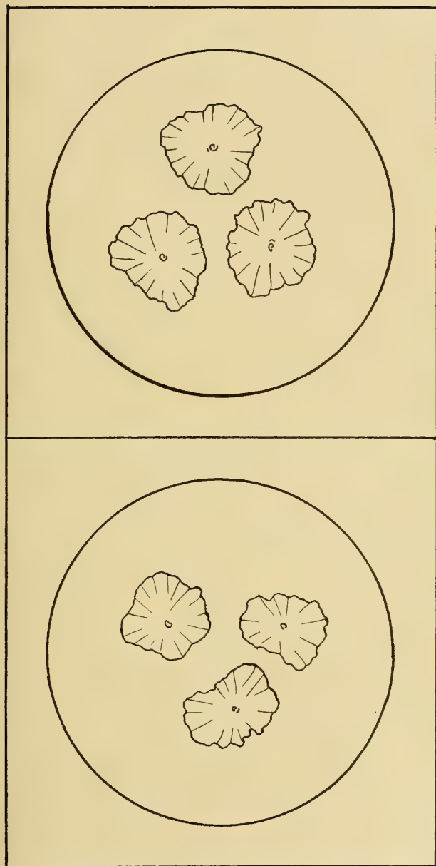
Fig. 2. — CHLORELLA VARIEGATA .
