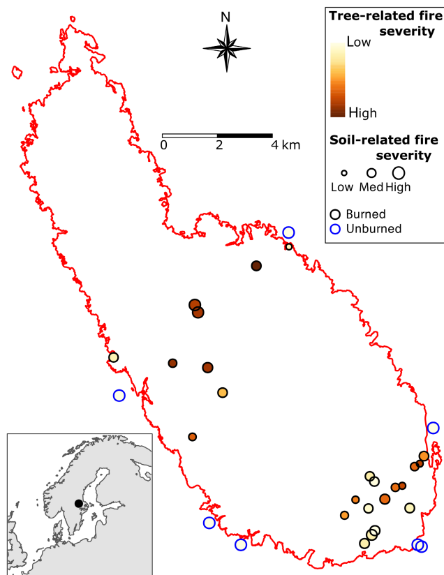
FIGURE 2 Map of the Västmanland burn that occurred in Sweden in 2014, and of the physical location of each of the 32 individual forest stands sampled in this study. Red contour line represents the fire boundary. Black outer line dots represent 25 individual burned stands and blue outer line dots represent the seven unburned reference stands. Circles corresponding to burned plots are colored according to tree-related fire severity (from yellow [low] to brown [high]) and sized according to soil-related fire severity. GPS coordinates for each stand are given in Table S1.
