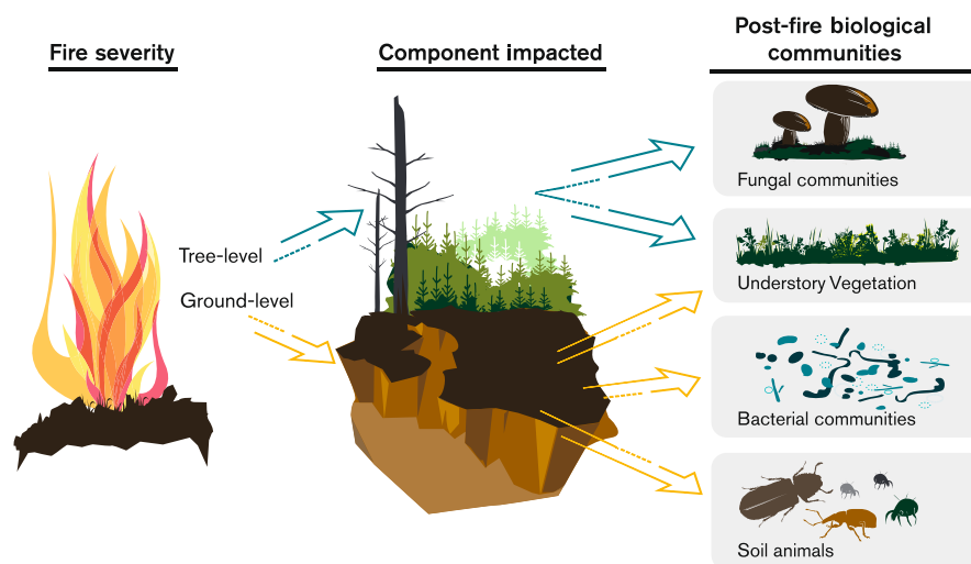
FIGURE 1 Conceptual diagram showing how we hypothesize that two separate fire severity gradients will affect biological communities: one aboveground gradient that is mainly attributed to damage of the trees and one gradient attributed to damage on the forest floor.
