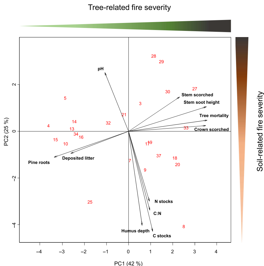
FIGURE 3 Principal component analysis (PCA) of aboveground and belowground variables that are indicative of tree-related fire severity and soil-related fire severity, respectively. The first two axes explaining the largest proportions of total variation (in parenthesis) are shown. Numbers represent forest stand IDs (Table S1). Mean values of each variable can be found in Table S4.
