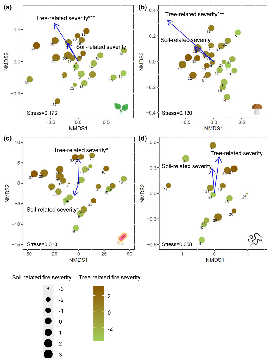
FIGURE 5 Ordination analysis of response variables displayed by NMDS for community composition of (a) understory vegetation, (b) soil fungi, (c) soil bacterial PLFAs, and (d) soil Nematoda. Vectors indicate the direction and magnitude of correlations of community assemblage with tree-related fire severity and soil-related fire severity indexes. Asterisks denote level of significant correlations (* p < 0.05 , ** p < 0.01 , and *** p < 0.001 ). Stress values shown at the bottom of each graph correspond to two dimensions ( k=2 ). Numbers represent forest stand IDs (Table S1).
