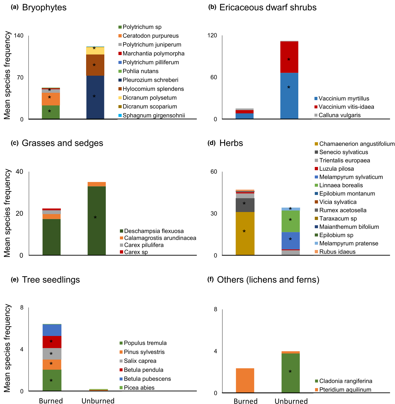
FIGURE 4 Mean frequency of species of (a) bryophytes, (b) ericaceous dwarf shrubs, (c) grasses and sedges, (d) herbs, (e) newly established tree seedlings, and (f) others (lichen and ferns) that are present in more than one stand in the understory of the burned and unburned forest stands. Asterisks indicate significant differences for individual species between burned and unburned forests (results of the statistical tests in Table S5).
