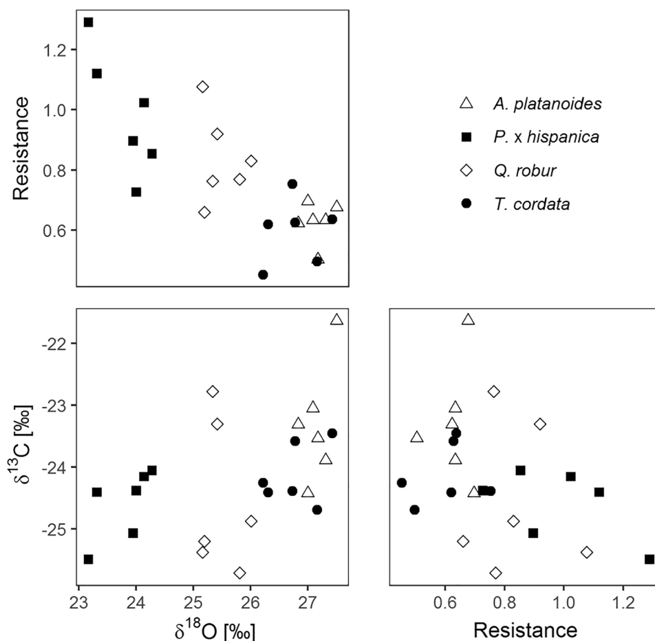
Fig. 6 Correlation between mean values (per tree, n_{\text{trees}}=6 ) of resistance (mean of the years 2003, 2011 and 2015), \delta^{13}\text{C} and \delta^{18}\text{O} (mean for 2000–2018)
