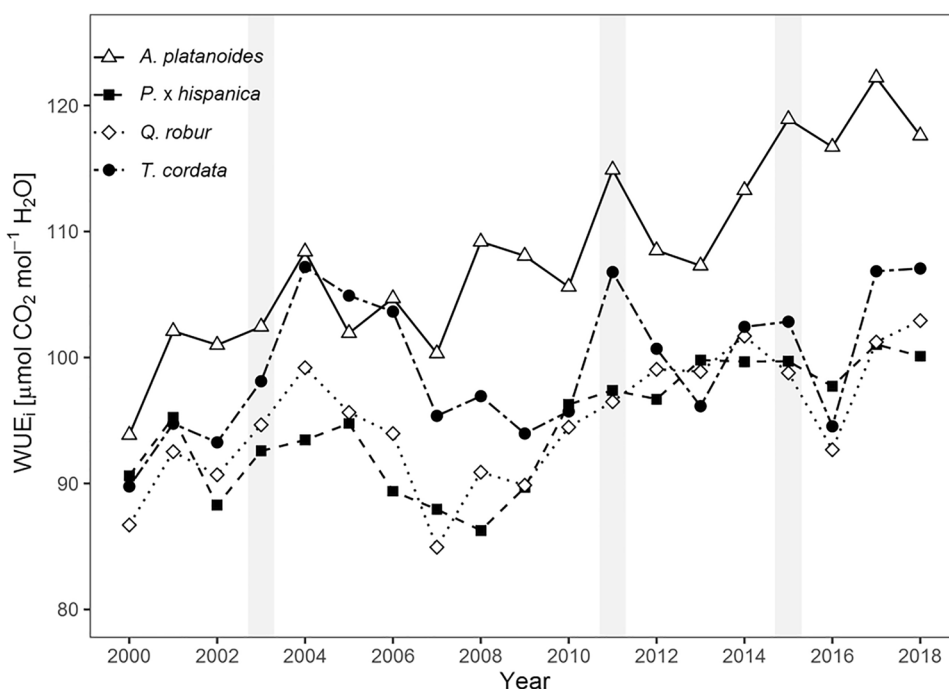
Fig. 2 Annual intrinsic water-use efficiency ( WUE_i ) for the time period 2000–2018. The three years with exceptional droughts (2003, 2011 and 2015) are highlighted by light grey vertical bars
