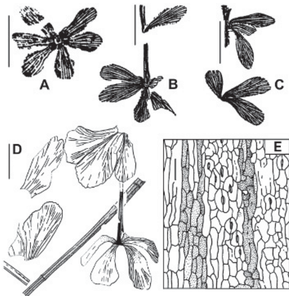
Figure 5. Permian sphenophylls of the Pechora Cis-Urals; Sphenophyllum comiense Tschirkova, emend. Naug., emend. nov. (A–E). A–C – canonic illustrations of Sphenophyllum comiense , published in ZALESSKY & TSCHIRKOVA (1938); B – lectotype, selected by NEUBURG (1964); D – the leafy stems, preserved together (after NAUGOLNYKH 2007, p. 116, fig. 46), spec. GIN 4851/298; E – epidermal structure of the leaf Sphenophyllum comiense , spec. GIN 4851/289B. Localities: Vorkuta River, left bank near the Ajachjaga River mouth, Ajachjaginskaya Subformation, outcrop 49, packet S (A–C); Vorkuta River, outcrop 37 (D); KhK-1155, depth 51.6 m (E). Scale bars = 1 cm (A–D); 50 \mu m (E).
