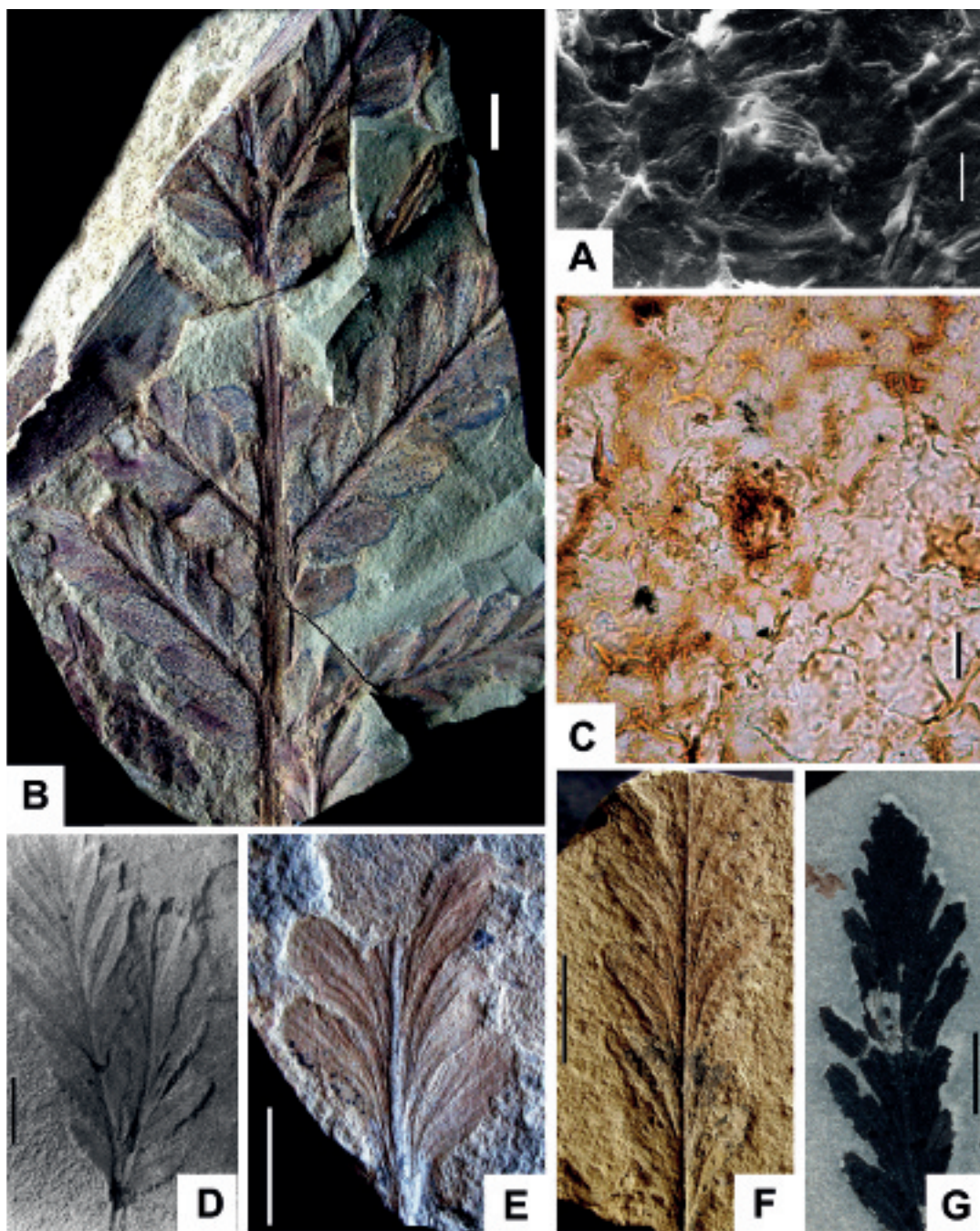
Figure 8. Permocallipteris artipinnata (Zalessky) Naug., comb. nov. Epidermal-cuticular structure (A, C) and general morphology of the leaves (B, D–G). A – the stoma with the well-visible lips-like guard cells, SEM, spec. 3773/368; B – middle part of the semi-adult frond with the intercalated pinnules, spec. UGM 2286; C – stoma with strongly cutinized guard cells, in light microscope, spec. 3773/368; D – apical part of the frond with pseudodichotomizing (overtopping) apex; spec. 3773/368, this specimen was macerated and used as a source of the cuticles shown here on Fig. 8A, C, and other cuticular preparations figured and published in previous work (NAUGOLNYKH 2007: Plates XXII–XXIV); E – middle part of the last order pinna with five completely preserved strongly decurrent pinnules, spec. 4856/508; F – almost completely preserved last order pinna, but without apex, spec. 4856/500; G – apical part of the last order pinna, spec. 3773(11)/328(92).
