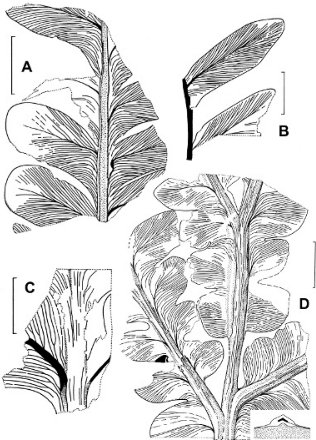
Figure 3. Permacallipteris adzvensis (Zalessky) Naug., comb. nov. Line tracings of general morphology of the leaves and details of their venation. A – middle part of the last order pinna, spec. 4851/239; B – part of pinna with relatively long lanceolate pinnules having slightly restricted bases, spec. 4851/241; C – details of venation in the basal part of the pinnule, spec. 4851/245; D – part of the large well-developed frond with pseudodichotomizing (overtopped) apex and intercalated pinnules, which are directly attached to the frond rachis and lack the clear midvein, spec. 4851/219. Localities: the Pechora Cis-Urals and Pechora Coal Basin; A – Loc. 708-391; B – Loc. 42K-159; C – Adzva River; D – NSK-210, depth 158.0 m. Scale bars = 1 cm.
