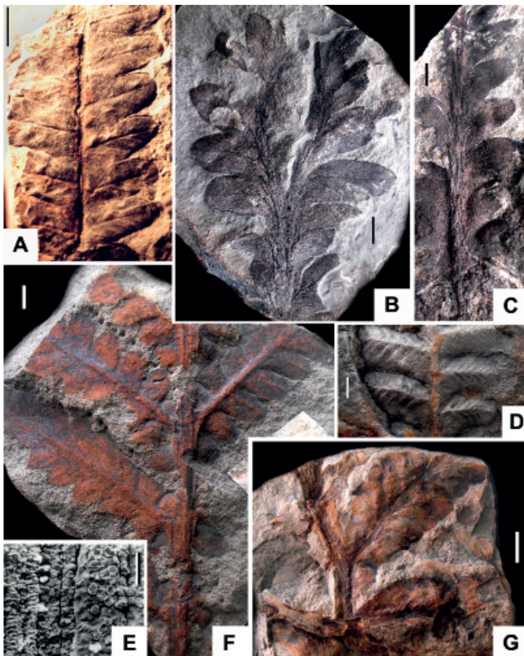
Figure 9. Permocallipteris wangenheimii (Fischer) Naug., comb. nov. A – the last order pinna, spec. GGM 469-1 FL-02589; B – the fork-shaped otopressed apex; same specimen was figured as Odontopteris tatarica Zalesky (ZALESSKY 1927: Plate XXXVII, Fig. 3, spec. TsNIGR 56/1543); C – the last order pinna, spec. TsNIGR 54/1543; counterpart of the same specimen – TsNIGR 55/1543; this specimen was figured as Odontopteris tatarica Zalesky (ZALESSKY 1927: Plate XXXVIII, Fig. 1); D – the young frond with unioherent venation; same specimen was figured as Callipteris uralensis Zalesky (ZALESSKY 1927: Plate V, Fig. 1); spec. TsNIGR 10/1543; E – anatomy (tracheids) of the frond rachis, spec. GGM 469-30 FL-026118 (for details see: NAUGOLNYKH 2002: Text-Fig. 5 A–D; Plates II–III); F – middle part of the well-developed frond, spec. TsNIGR 7/1543 (same specimen was figured by KUTORGA 1844: Plate V, Fig. 1, as Pecopteris principalis Kutorga); G – lower part of the adult frond with unioherent pinna, spec. TsNIGR 14/1543; same specimen was figured in ZALESSKY 1927: Plate VI, Fig. 4).
