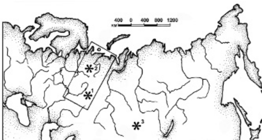
Figure 1. Geographical position of the main localities cited in the text. 1 – the Middle Cis-Urals (localities: Molebka, Krutaya Katushka-1, Krutaya Katushka-2, Krasnaya Glinka, Matveevo, Taezhnoe-1, Taezhnoe-2, Chekarda-1, Yulaevo, Mazuevka, Rakhmangulovo); 2 – Pechora Cis-Urals and Pechora Coal Basin; 3 – Kuznetsk basin.
