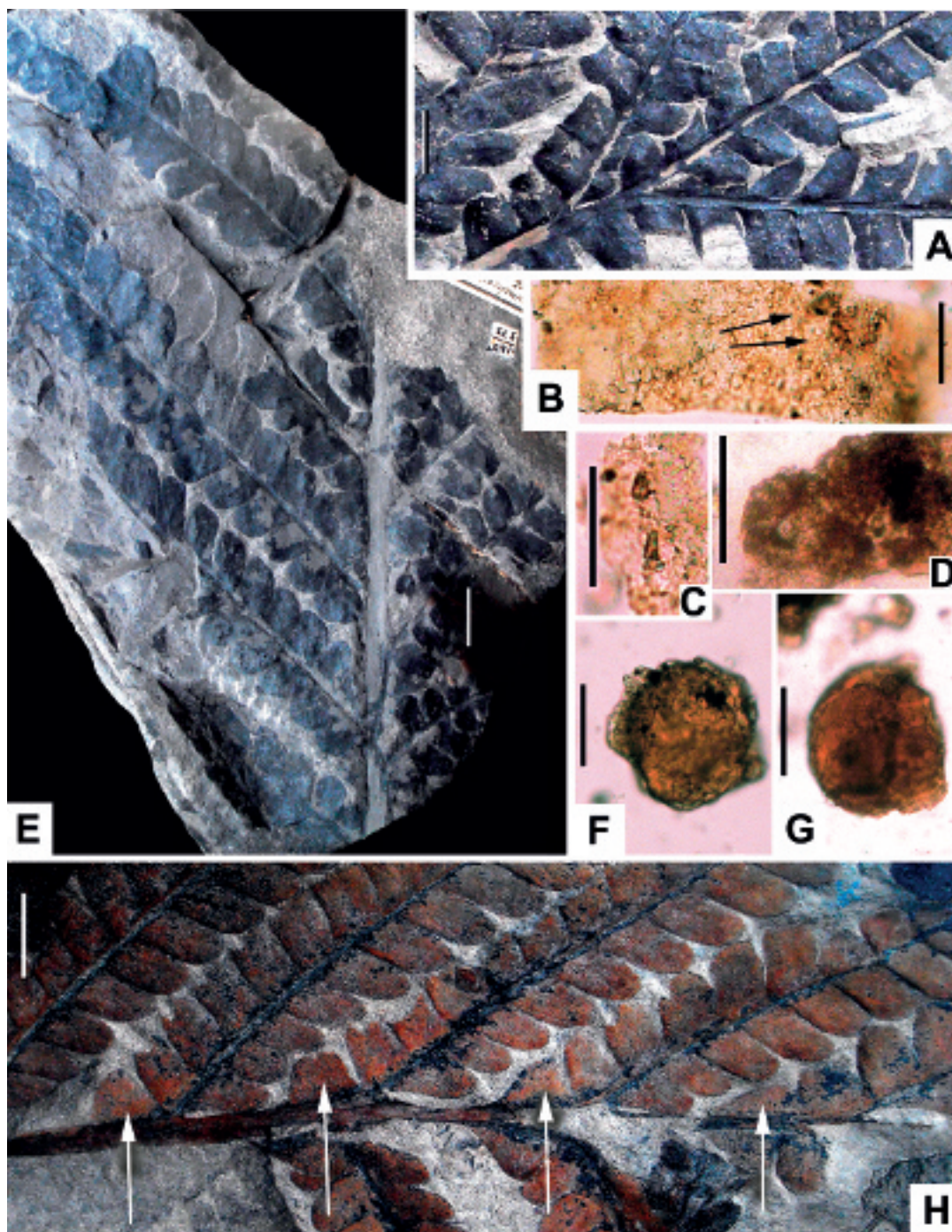
Figure 10. Permcallipteris zeillerii (Zalessky) Naug., comb. nov. A – apical part of the well-developed frond, lectotype, spec. TsNIGR 72/573 (figured in ZALESSKY 1918: Plate XLV, Fig. 2); B–D, F, G – cuticular structure, spec. TsNIGR 180/573; B – two neighboring resin bodies (marked by arrows); C – two unicellular hairs of conic shape; F, G – the resin bodies of round (F) and ovoid (G) shape; D – two neighboring stomata with thick proximal cutinization of the subsidiary cells; E – the specimen macerated (the cuticle preparations are shown here Fig. 10 B–D, F, G, TsNIGR 180/573); H – adult frond with well-developed intercalated pinnules (marked by arrows), spec. 73/572 (same specimen was figured in ZALESSKY 1918: Plate XLV, Fig. 1).
