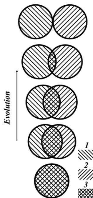
Figure 29. Diagram of synchronous divergent evolution of water-conducting and strengthening subsystems of the secondary wood. 1 – water-conducting subsystem; 2 – strengthening subsystem; 3 – tracheidal system/subsystem with equally combined water-conducting and strengthening functions.
