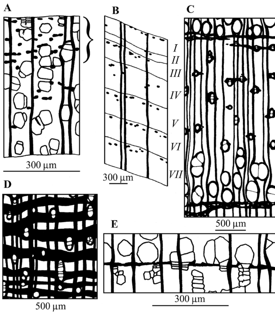
Figure 22. Patterns of the living constituents of the cross-sectioned SHWs. A – Alnus incana (L.) Moench; B – Fitzroya patagonica Hook. f.; C – Fraxinus excelsior L.; D – Ficus carica L.; E – Populus tremula L. Brace – outer 1/3 growth ring; I–VII – successive growth rings.
