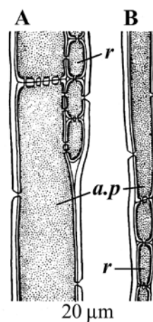
Figure 23. Contacts between axial and ray parenchyma of the SHW of Alnus incana (L.) Moench. A – lateral contact of the axial parenchyma strand; B – terminal contact of the axial parenchyma strand. a.p – axial parenchyma; r – ray.
