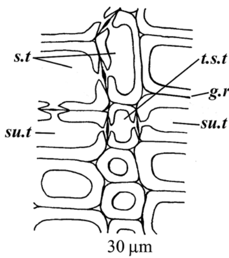
Figure 19. Summer / spring wood boundary in SVW of Ginkgo biloba L. g.r – growth ring boundary; s.t – spring wood tracheids; su.t – summer wood tracheids; t.s.t – terminal part of spring wood tracheid intruding into the mass of summer wood tracheids.
