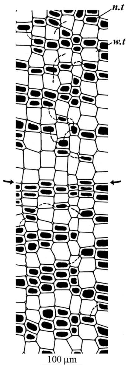
Figure 20. Patterns of narrow and wide tracheids in the cross-sectioned SVW of Ginkgo biloba L. n.t – narrower thin tracheid; w.t – wider thick tracheid; arrow – growth-ring boundary; dotted line – intermediated communications between the tracheids.
