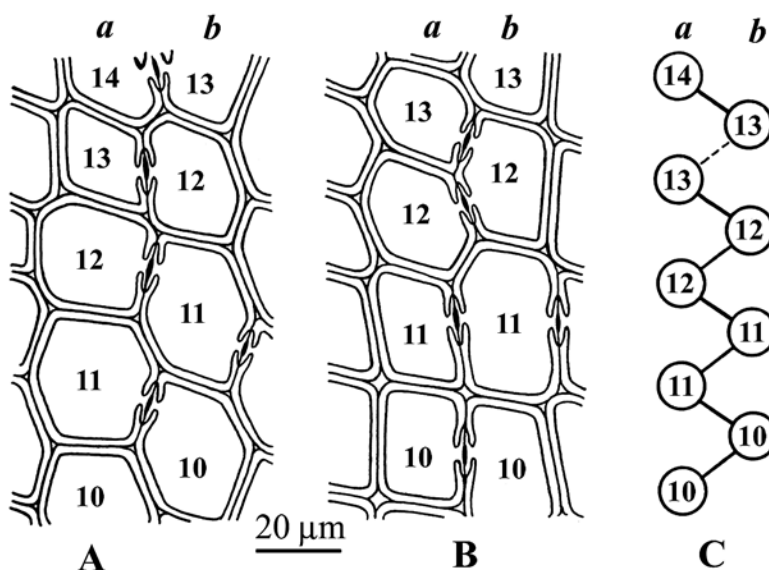
Figure 12. Radial communications between tracheids of the spring wood in Thuja occidentalis L. A, B – serially cross-sectioned wood; C – diagram of communications. a , b – contiguous rows of the tracheids; arabics – numbers of the successive tracheids in a row.
