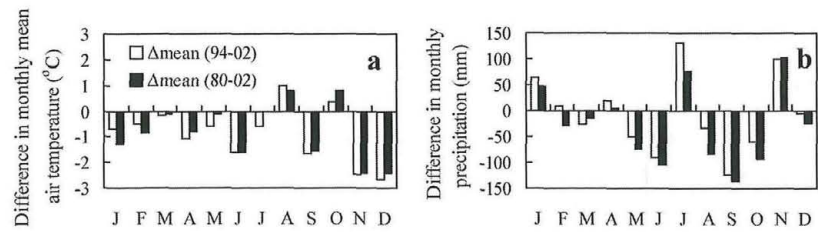
Fig. 1. Difference in monthly mean air temperature (a) and precipitation (b) between 1995 and the mean of 1994-2002 (white block) and 1980-2002 (black block). Air temperature data of 1994-2002 come from the study site, observed at 25 m height on tower. Other datasets come from the Takayama Research Station, ca. 500 m north of the study site.
