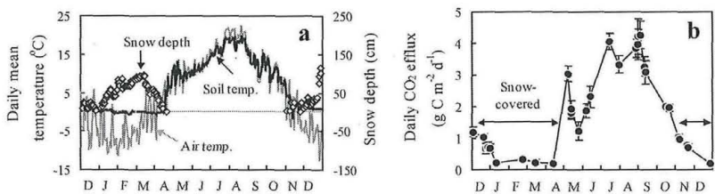
Fig. 2. Seasonal changes in (a) air and soil temperature and snow depth, and (b) daily CO 2 -C efflux from Dec. 1994 to Dec. 1995 in Takayama. Air temperature at 25 m height observed on the tower, and soil temperature at 1-cm measured near the study site of efflux. Snow depth data come from the Takayama Research Station. C-efflux measured with the open-flow IRGA method from soil surface (snow-free season) and snow surface (snow-covered season). Error bars in (b) represent the standard deviation (n=4) of efflux.
