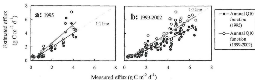
Fig. 4. Relationship between measured and estimated daily CO 2 -C effluxes based on the annual Q 10 function derived from 1995 dataset and by 1999–2002 datasets. (a) 1995 dataset (n=30) of this study, for annual Q 10 function (1995): slope = 1.01, intercept = -0.04, r 2 = 0.77, and for annual Q 10 function: slope = 1.33, intercept = -0.12, r 2 = 0.76; and (b) 1999–2002 dataset (n=60) of MO et al. (2004), for annual Q 10 function (1995): slope = 0.75, intercept = 0.07, r 2 = 0.82, and for annual Q 10 function: slope = 0.99, intercept = 0.01, r 2 = 0.82. The regression lines are all significant (P < 0.001).
