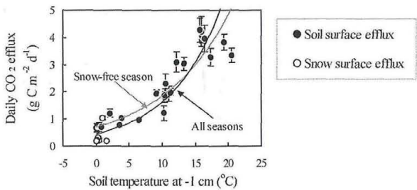
Fig. 3. Relationship of daily CO 2 -C efflux and daily mean soil temperature at -1 cm. Error bars represent the standard deviation (n=4). Solid line represents the regression line for all seasons (including snow-covered season), and dash line represents the regression line for snow-free season. The regression equations are shown in Table 2.
