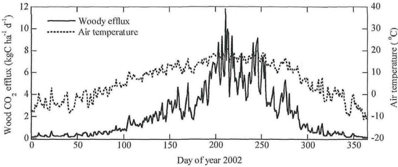
Fig. 3. Relationship between wood CO 2 efflux and air temperature.
