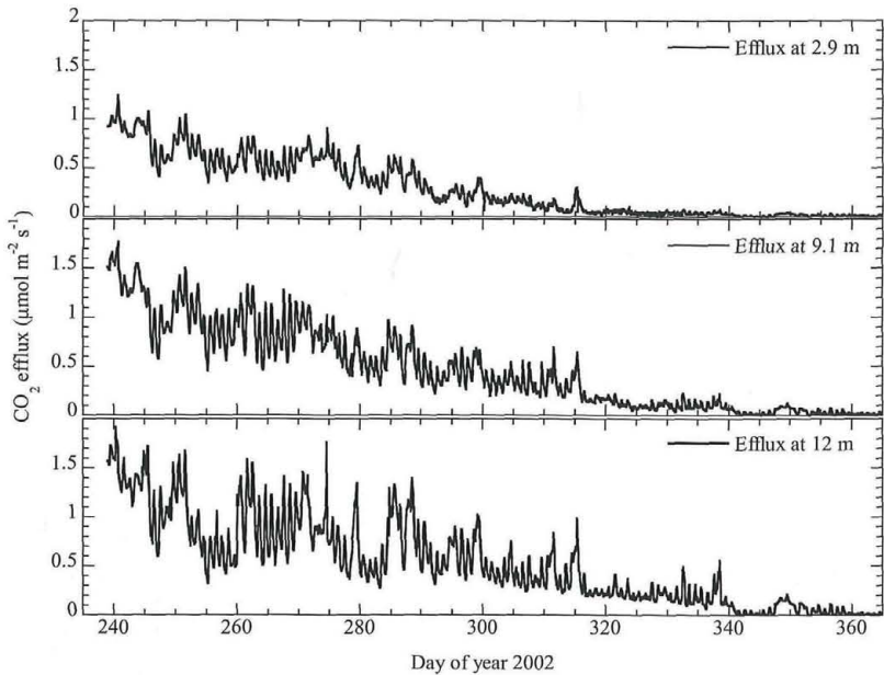
Fig. 1. Seasonal change in wood CO 2 efflux at different heights of stem on unit surface area basis.
