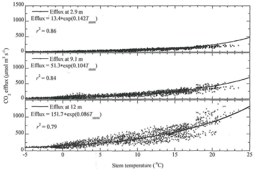
Fig. 2. Temperature response function of wood CO 2 efflux.
