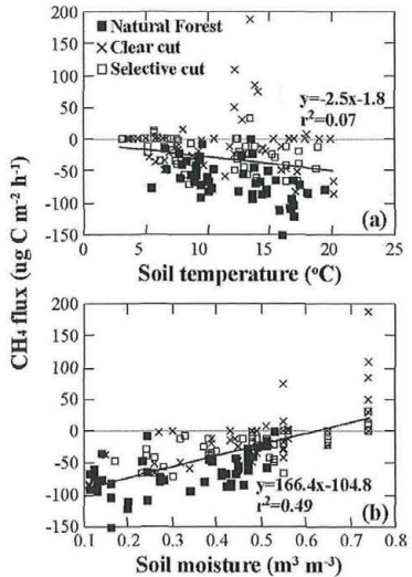
Fig. 4. Relationship between CH 4 flux and a) soil temperature and b) moisture.
